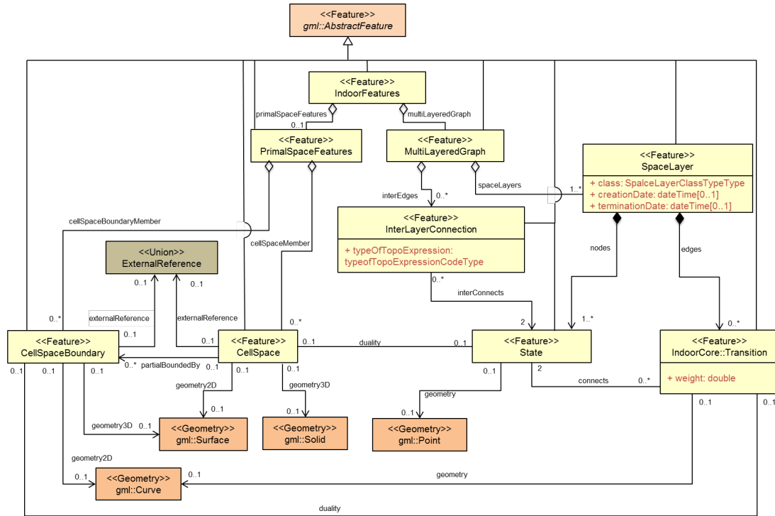
Figure 21: UML diagram of IndoorGML's core module(Multi-Layered Space Model)
