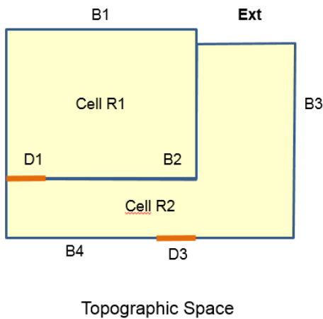
Figure 4-a. Primal space
