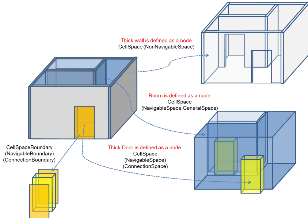
b) Example for Thick Door Model
