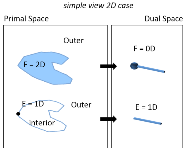
Figure 3-b: 2D Primal space case
