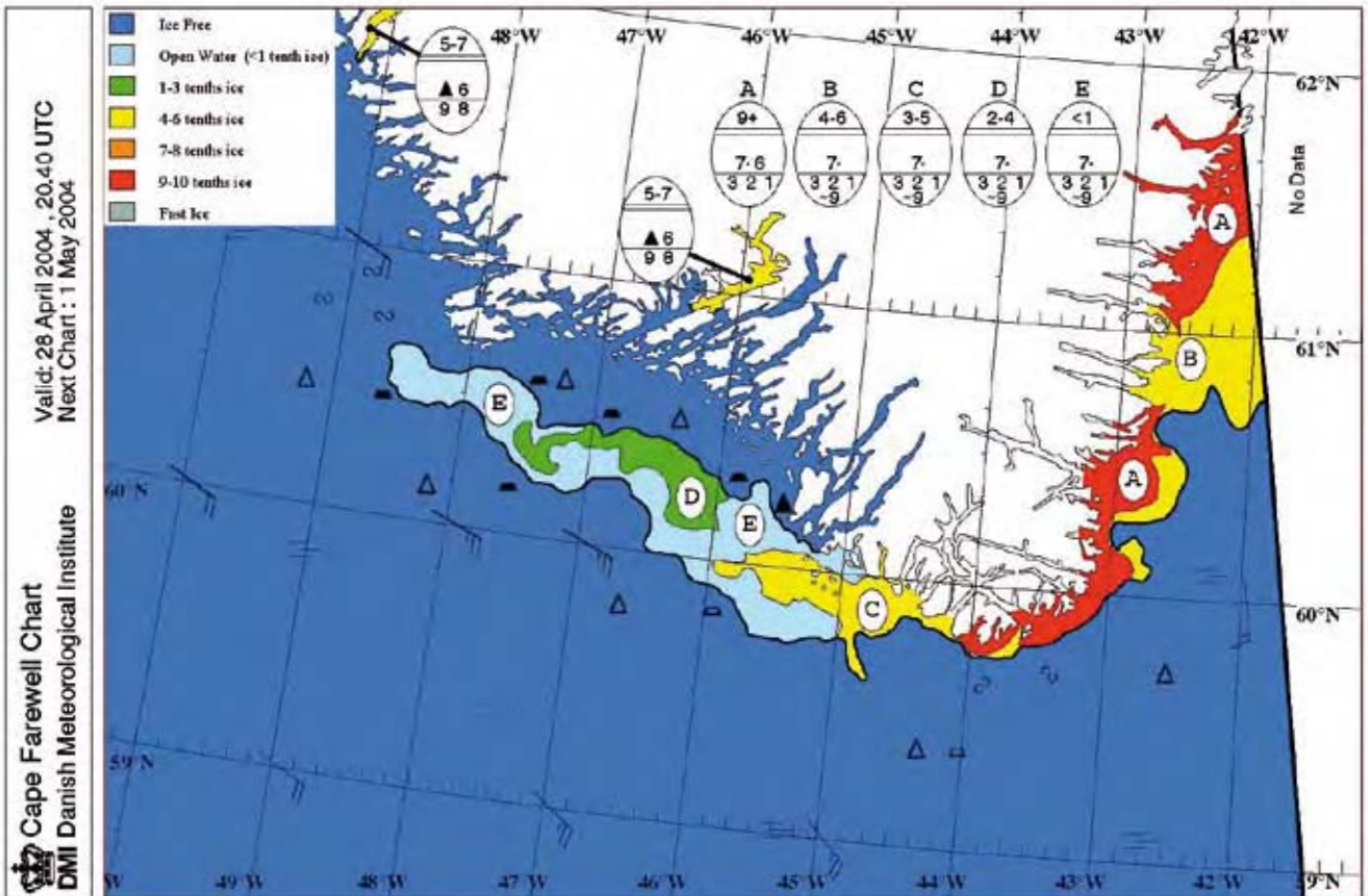
Figure III-4 – Cape Farewell ice chart for 28 April 2004.
