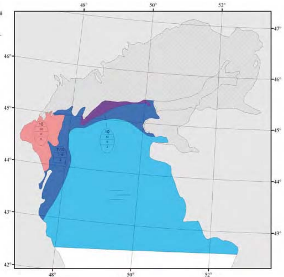
Figure X-6 – Annotated visible imagery from MODIS EOS Terra (mosaic of channels 1, 2 and 4) and detailed ice charts for the Caspian Sea for 14–15 February 2005.
