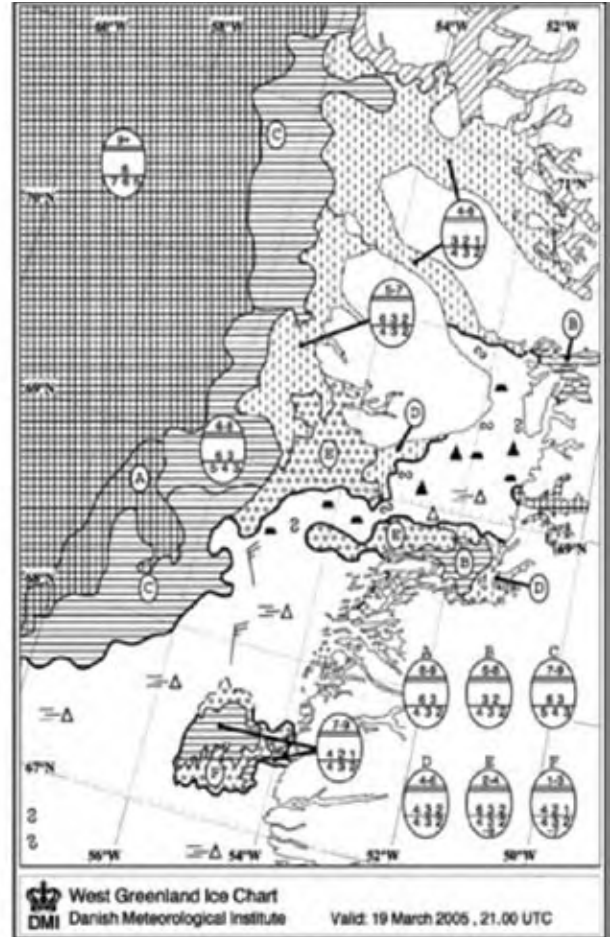
Figure III-3 – West Greenland ice chart for 19 March 2005.
