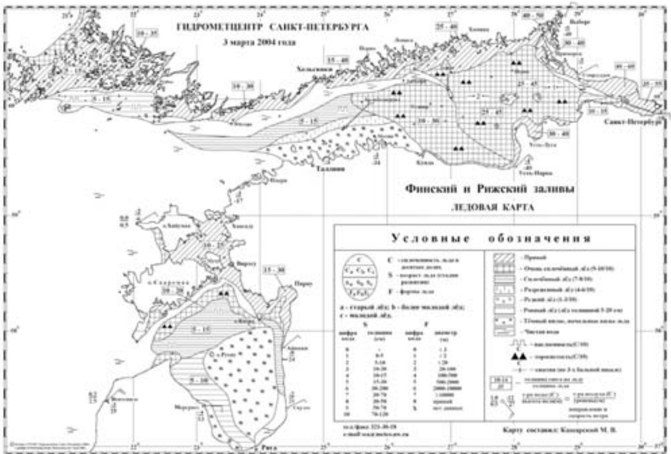
Figure X-7 – Daily ice chart for the gulfs of Finland and Riga for 3 March 2004.
