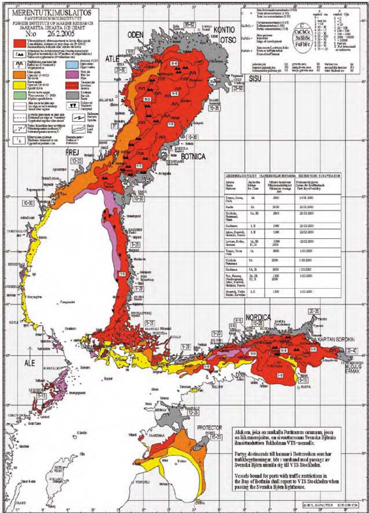
Figure V-1 – Daily ice chart for the Baltic Sea for 26 February 2005.
