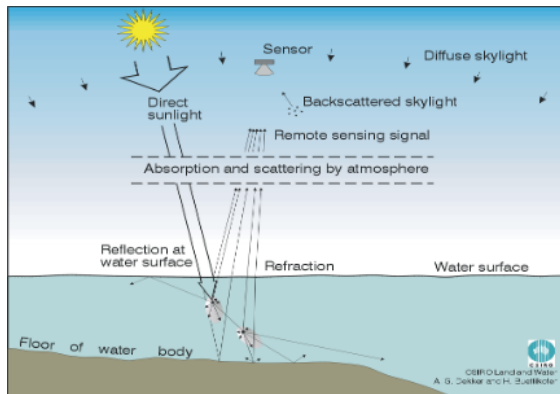
Figure 1. A. Schematic of light propagation in the atmosphere and underwater (Courtesy of A. Dekker and H. Buettikofer, CSIRO). B. Aerial photo of the Daintree coastal region showing the change of water colour as a function of in-water constituents (e.g., highest sediment content closest to shore) and the illumination conditions (e.g., impact of clouds) (Photo credit: K. Oubelkheir).
