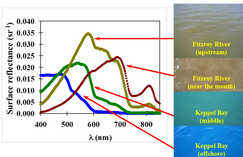
Figure 2. Left: Examples of surface reflectance spectra in contrasted situations (from the highly turbid waters of the Fitzroy Estuary to the clear blue waters offshore in nearby Keppel Bay). Right: Corresponding water surface photos (Photo credit: K. Oubelkheir).
