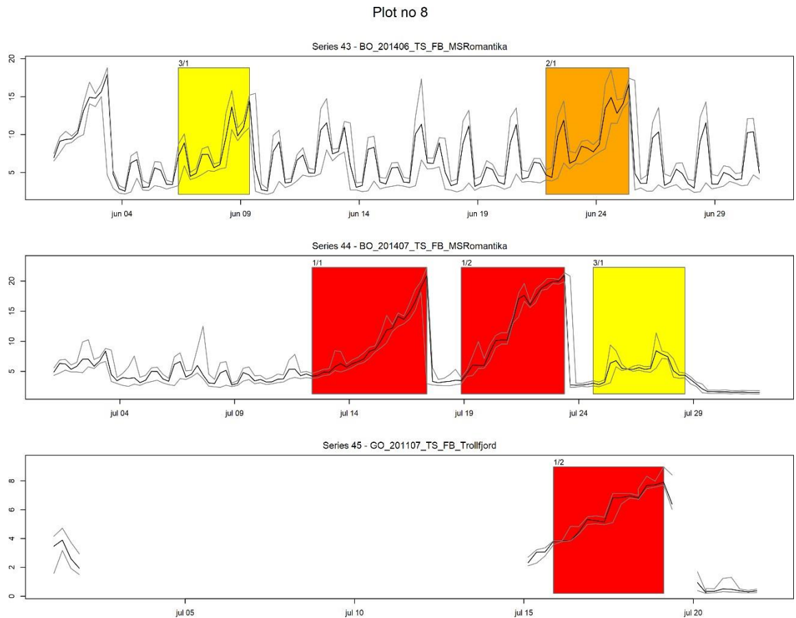
Figure 6 Biofouling indication. The time series shown are 6-hour means of Chl a fluorescence, and the yellow-, orange and red-coloured areas indicate where the mathematical properties of the time series indicate possible fouling. The indication is used together with expert judgement.
