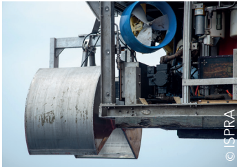
Grab sampler mounted on a Class II ROV
