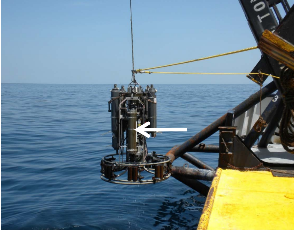
Figure 2-1. A profiling Sea-Bird CTD (conductivity, temperature, and depth) mounted on a rosette with Niskin bottles is recovered during a cruise aboard the RV OCEAN VERITAS following the 2010 Deepwater Horizon incident (photo courtesy of Mark Bushnell).
