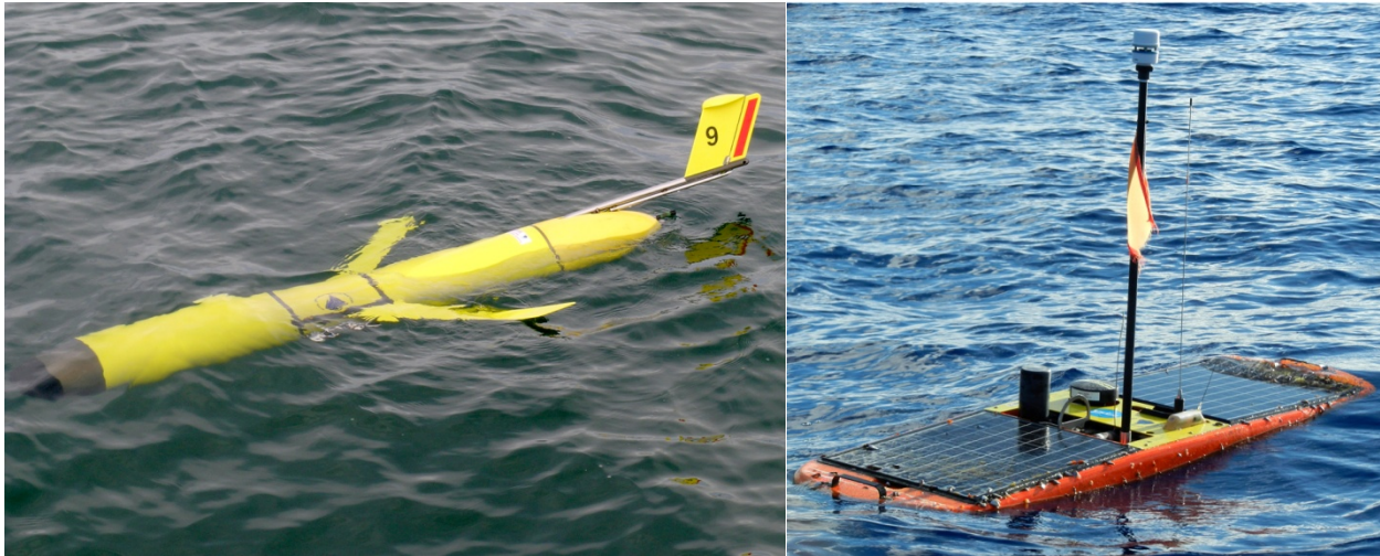
Figure 2-7. WebbGlider Profiler 3-D (L) and Wave Glider (R) (photo courtesy of Dave Fratantoni, Ph.D./Horizon Marine, Inc.).
