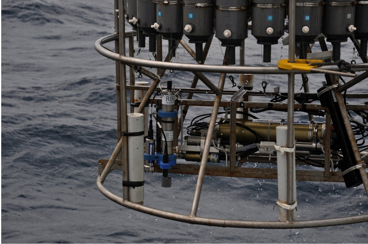
Figure 2-9. This CTD/bottle rosette shows the use of both Sea-Bird and RBR sensors (photo courtesy of Igor Shkvorets/RBR).
