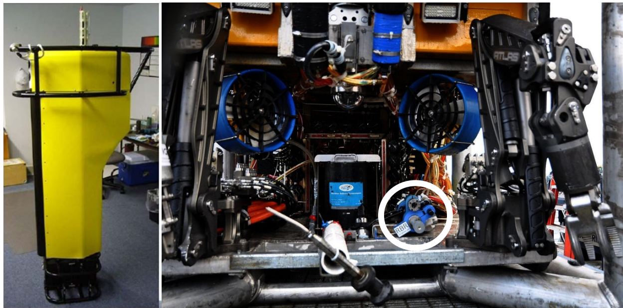
Figure 2-8. WET Labs AMP C100 In-Situ Profiler (courtesy of WET Labs) (L); RBR CTD sensor on an Oceaneering ROV (R) (photo courtesy of Igor Shkovorets/RBR).
