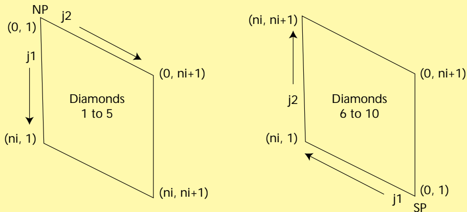
Figure 7. Grid-point indices for a northern (left) and southern (right) diamond.
