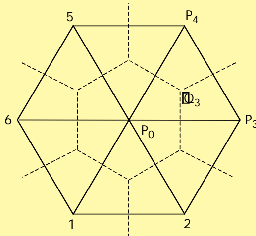
Figure 10. Hexagon connected to a grid-point of the triangular mesh.
