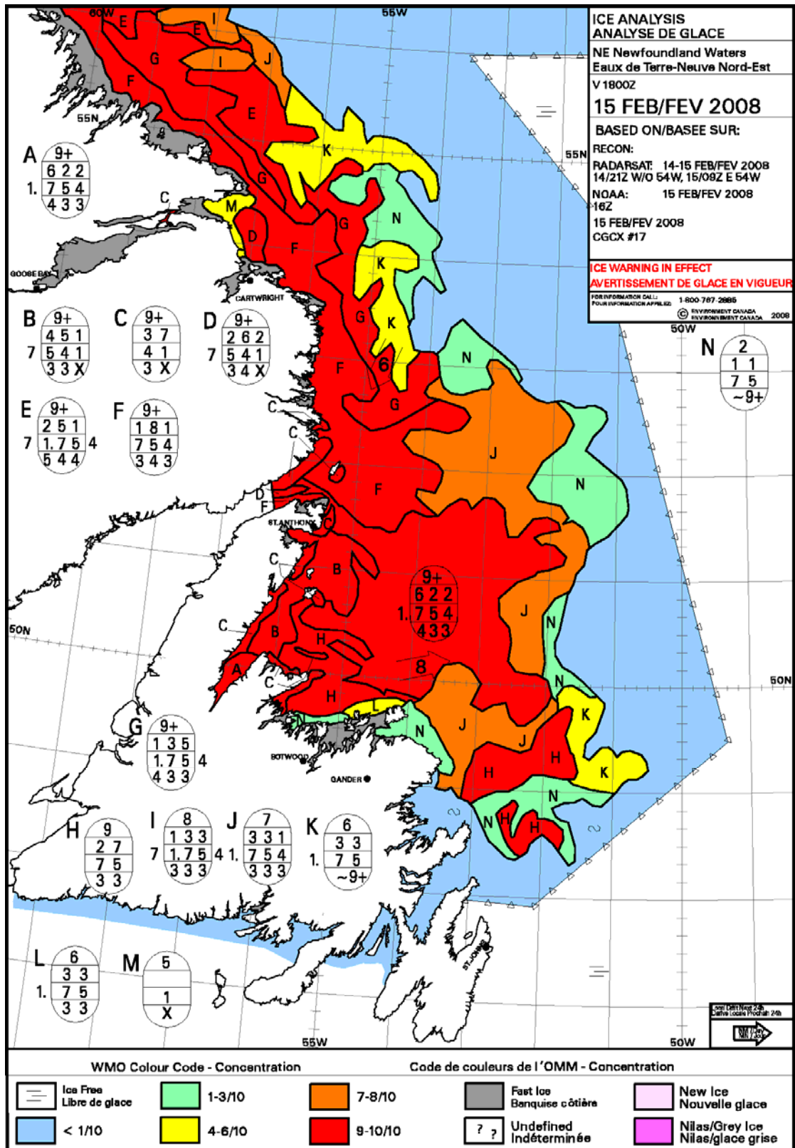
Figure I-3 – Daily Ice analysis chart for the Canadian East Coast for 15 February 2008.
