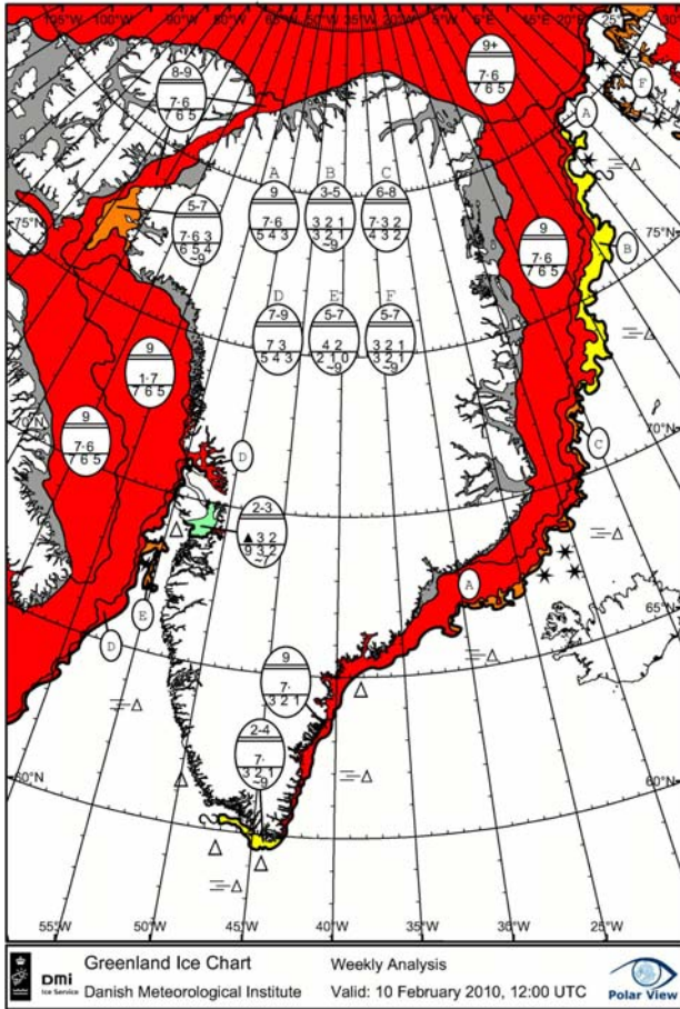
Figure III-2 – Weekly ice analysis for Greenland waters, 10 February 2010
