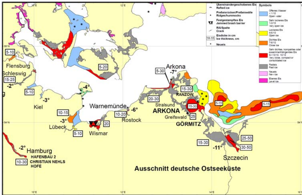
Figure VI-2 – German Baltic Sea coast chart, 31 January 2010.
