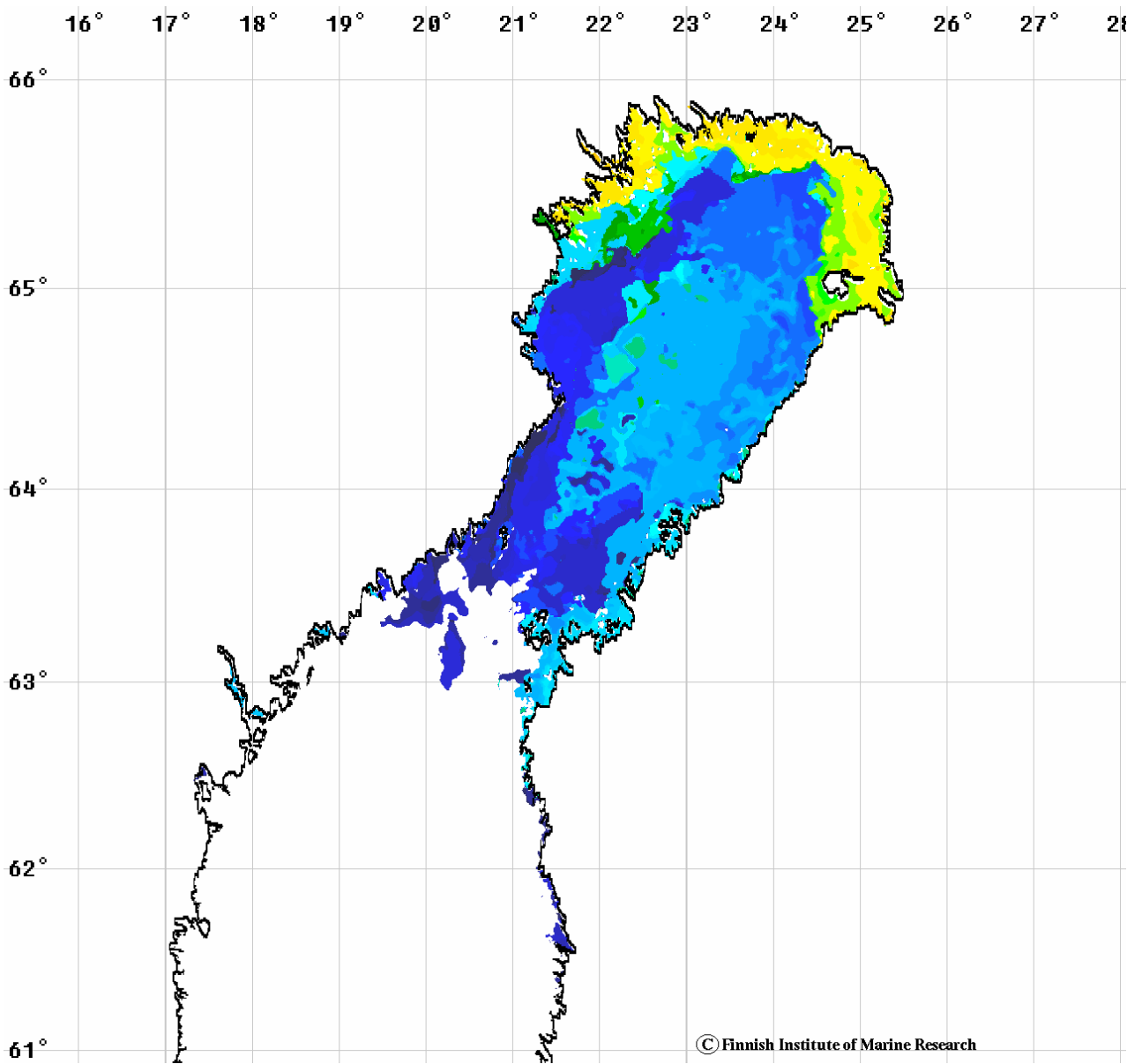
Figure V-2 – Example of high-resolution ice thickness map on 23 March 2008.
