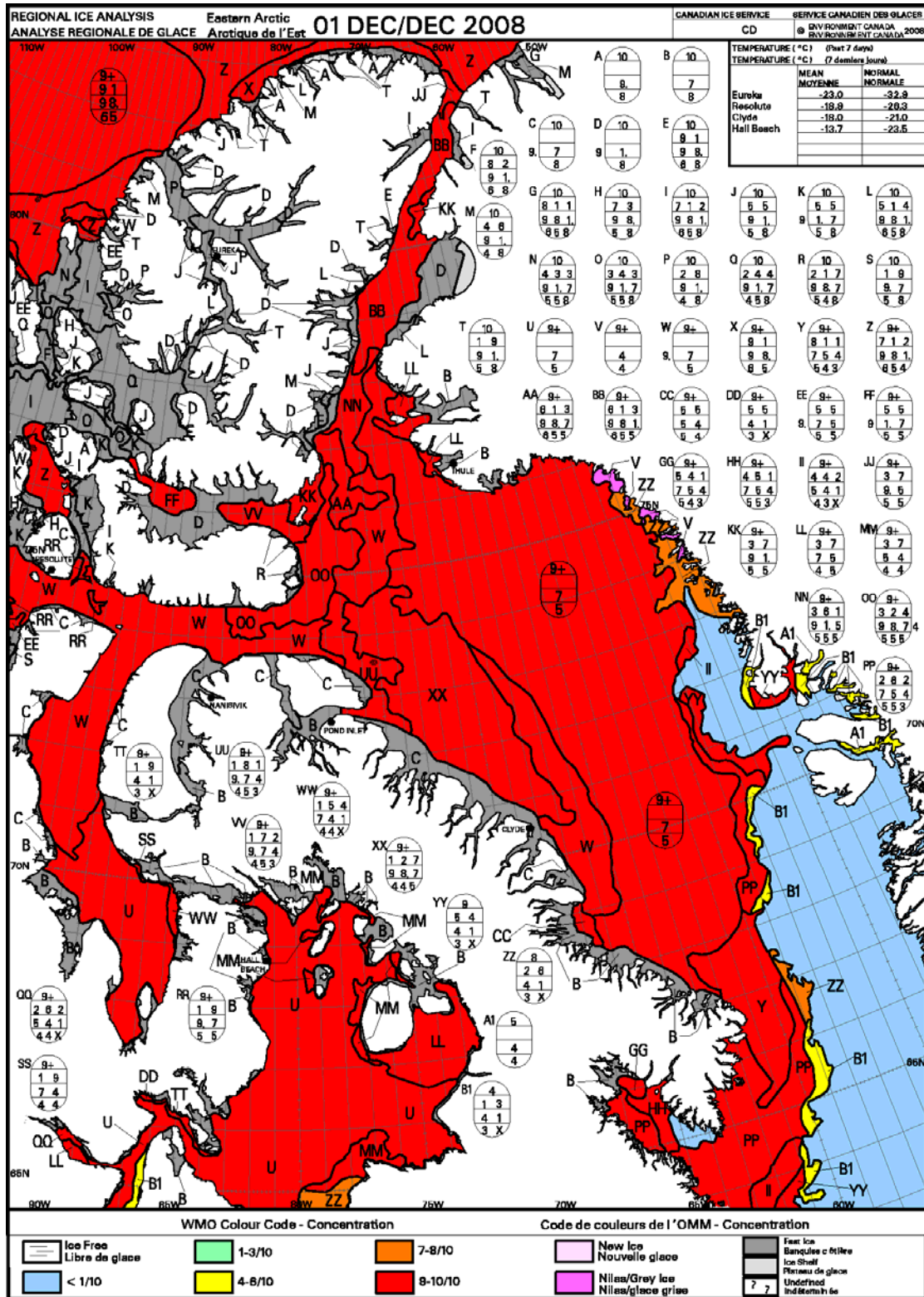
Figure I-1 – Regional Ice chart for the Eastern Arctic for 1 December 2008.
