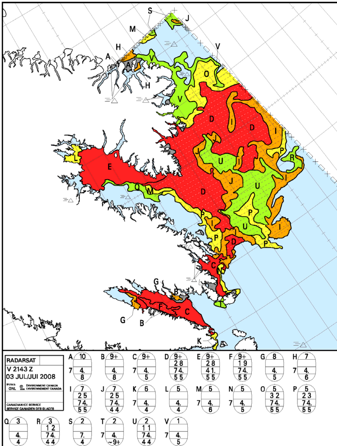
Figure I-5 – Image analysis chart for southern Davis Strait for 3 July 2008.
