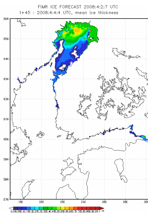
Figure V-3 – Examples of Finnish ice forecasts (0h and +45h)
