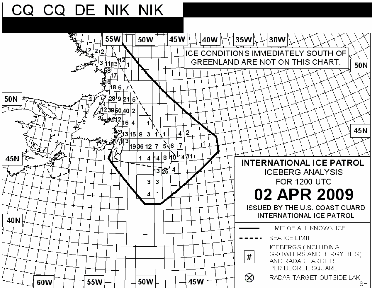
Figure XII-1 – Iceberg chart produced by the US Coast Guard International Ice Patrol for 2 April 2009.
