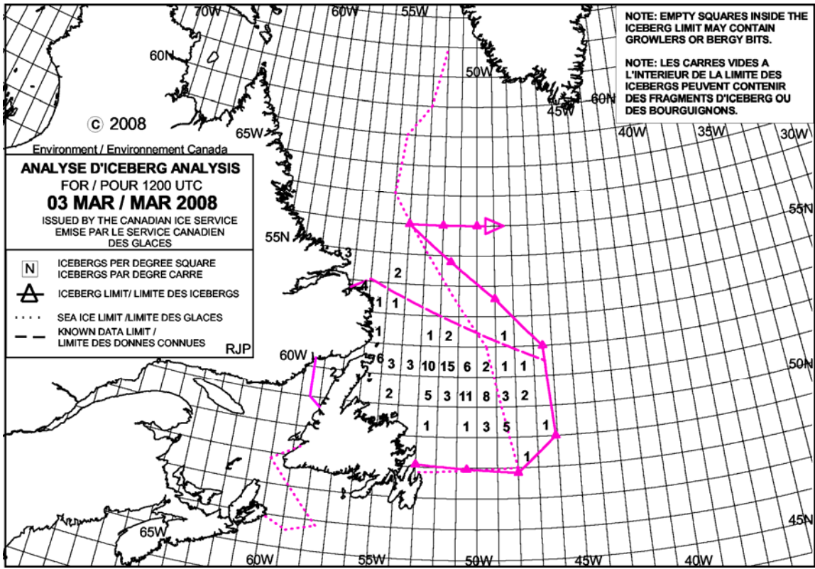
Figure I-2 – Daily Iceberg Analysis chart for the Canadian East Coast for 3 March 2008
