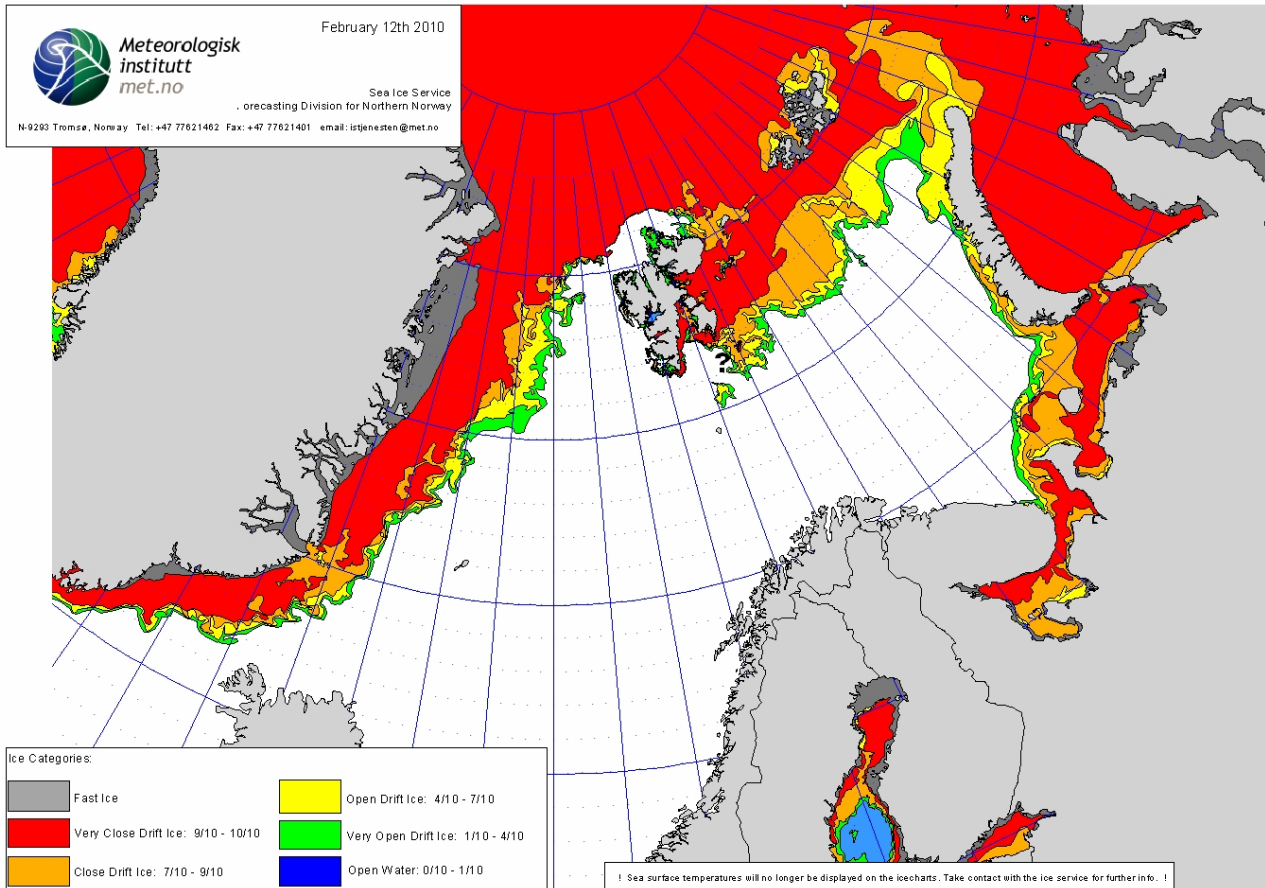
Figure VIII-1 – Daily ice chart for the Atlantic sector of the Arctic for 12 February 2010.
