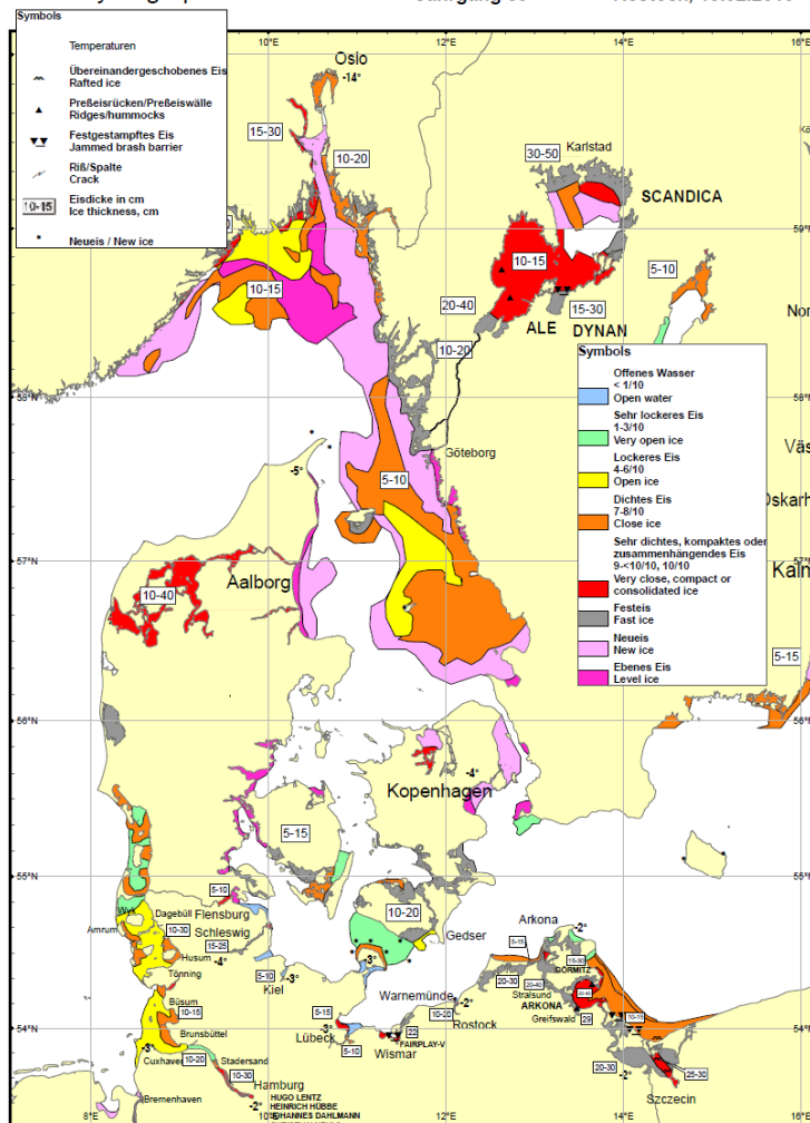
Figure VI-3 – Western Baltic Sea area and North Sea coast ice chart for 13 February 2010.
