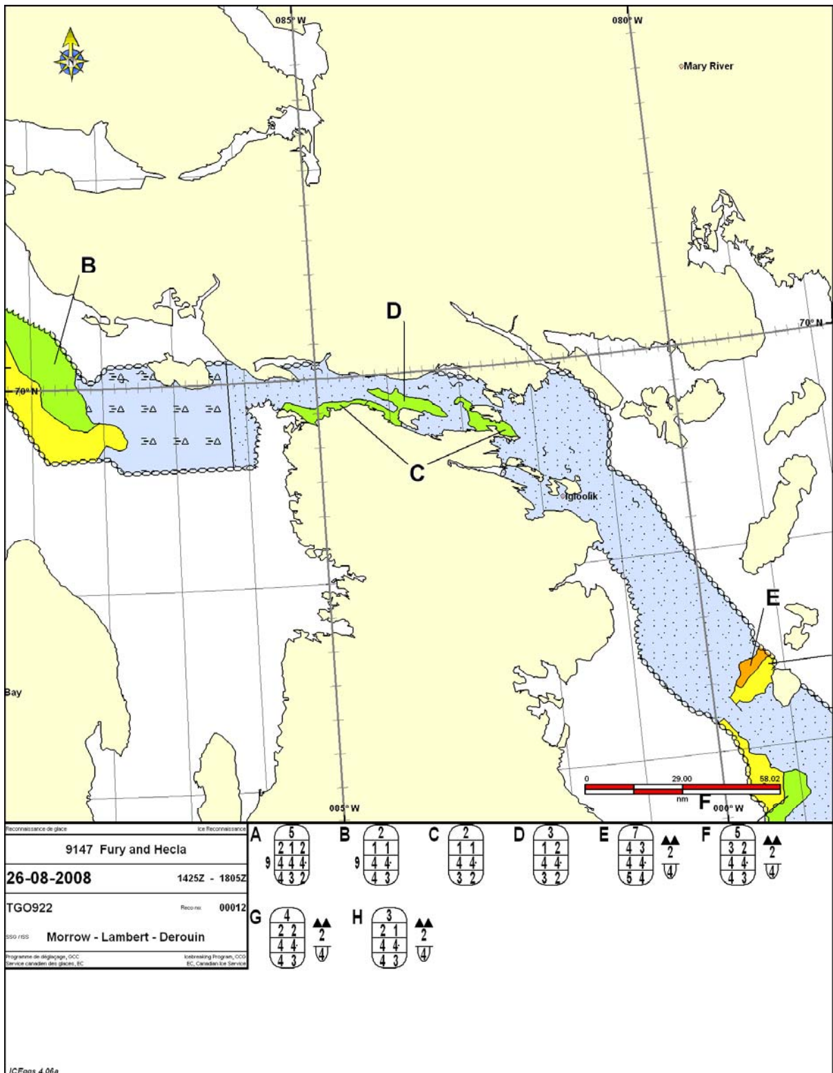
Figure I-4 – Ice Reconnaissance chart for Fury and Hecla for 26 August 2008.
