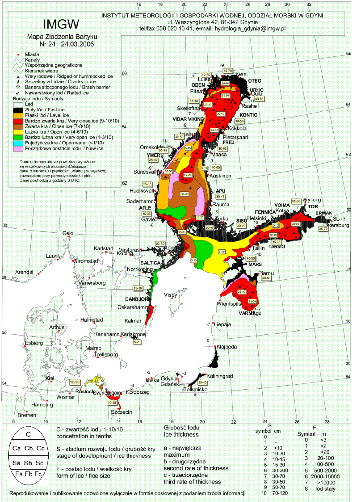
Figure IX-1 – Ice chart for the Baltic Sea on 24 March 2006.
