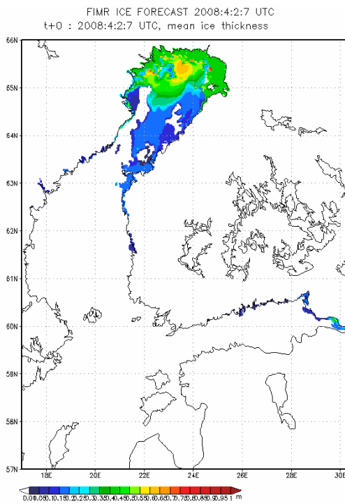
Figure V-3 – Examples of Finnish ice forecasts (0h and +45h)
