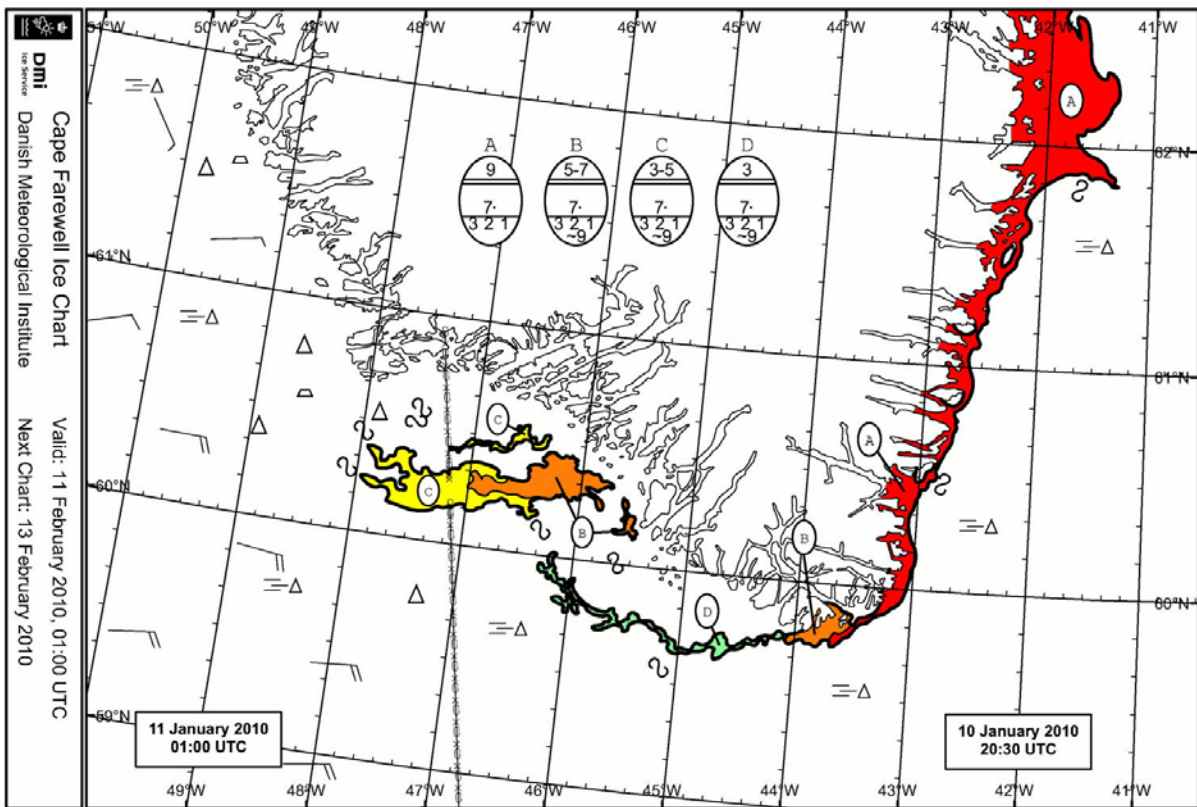
Figure III-4 – Cape Farewell ice chart for 11 February 01:00 2010.
