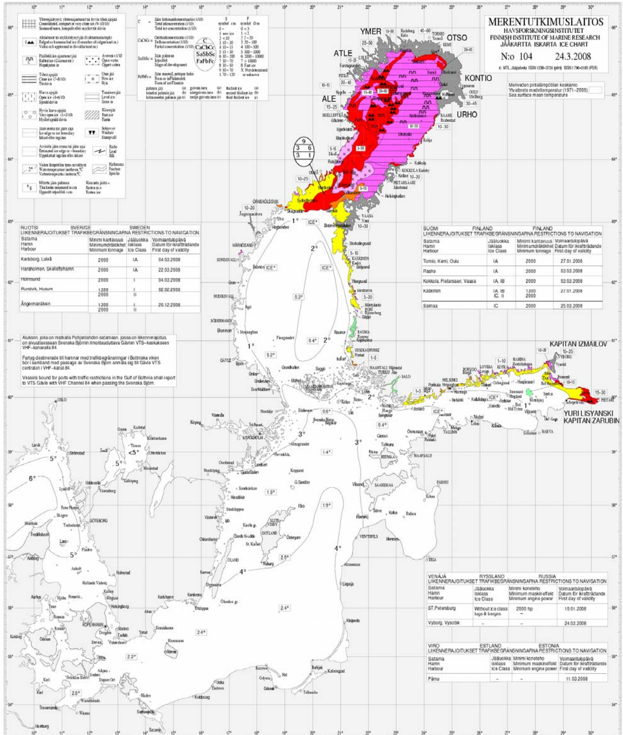
Figure V-1 – Example of Finnish ice chart on 24 March 2008.
