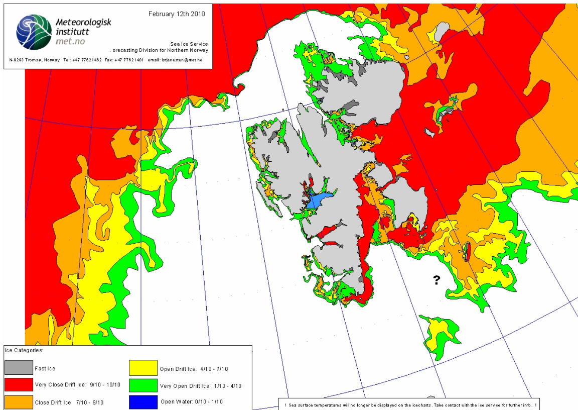
Figure VIII-2 – High-resolution ice chart for the Svalbard area for 12 February 2010.
