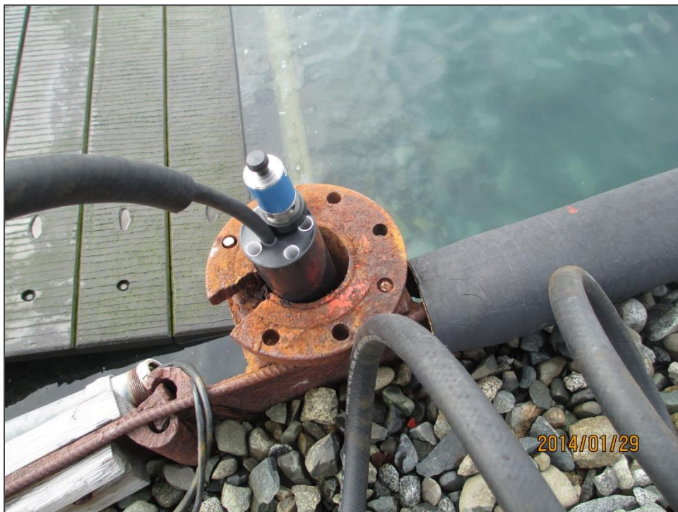
Figure 2-5. An Aanderaa 5218 pressure sensor is lowered into a protective well, providing single point, non-directional wave observations. (Photo courtesy of Richard Butler/Aanderaa)
