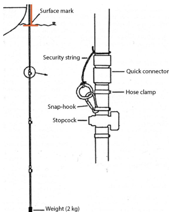
Figure 6. Hose-sampler dividable into segments for integrated samples of the water column (Lindahl 1986). Note the surface mark and the additional section of hose (marked in red), which must be added to the length (5m) of the first segment to cover the distance from the sea surface to the deck of the boat.
