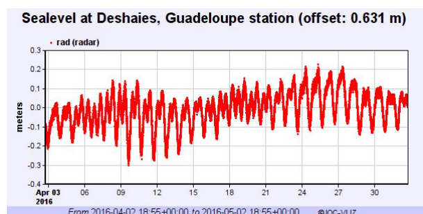
Figure 3. 30 days of data from the Deshaies, Guadeloupe station. The sensor is a guided wave radar and is operated by the IPGP in close collaboration with SHOM.
