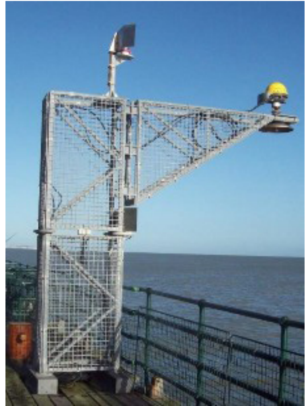
Figure 1. WaveRadar REX on Deal Pier © Canterbury City Council
