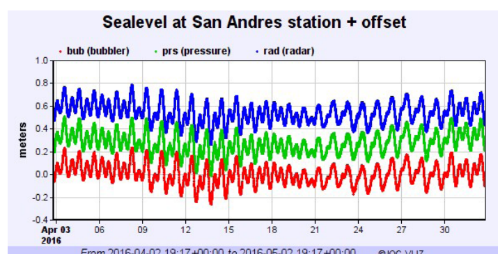
Figure 5. 30 days of data from the San Andres, Colombia sea level station operated by the UHSLC in close collaboration with the Colombian Navy. The data from the radar compares favorably with the data from the bubbler and the pressure sensor.
