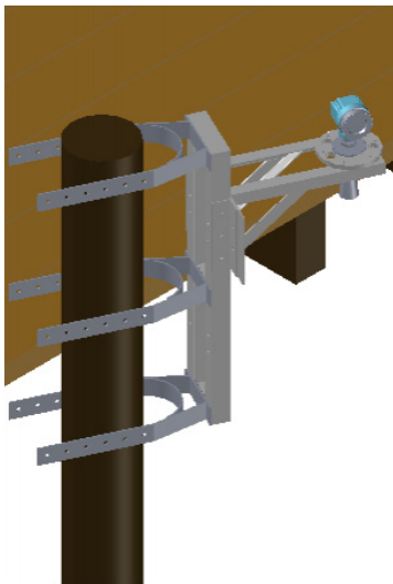
PILING CONCEPT WITH CONJUGATE RAILING BRACKET AND REDESIGNED PILE CLAMPS
