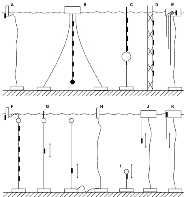
Figure 5.2.3. Mooring designs
