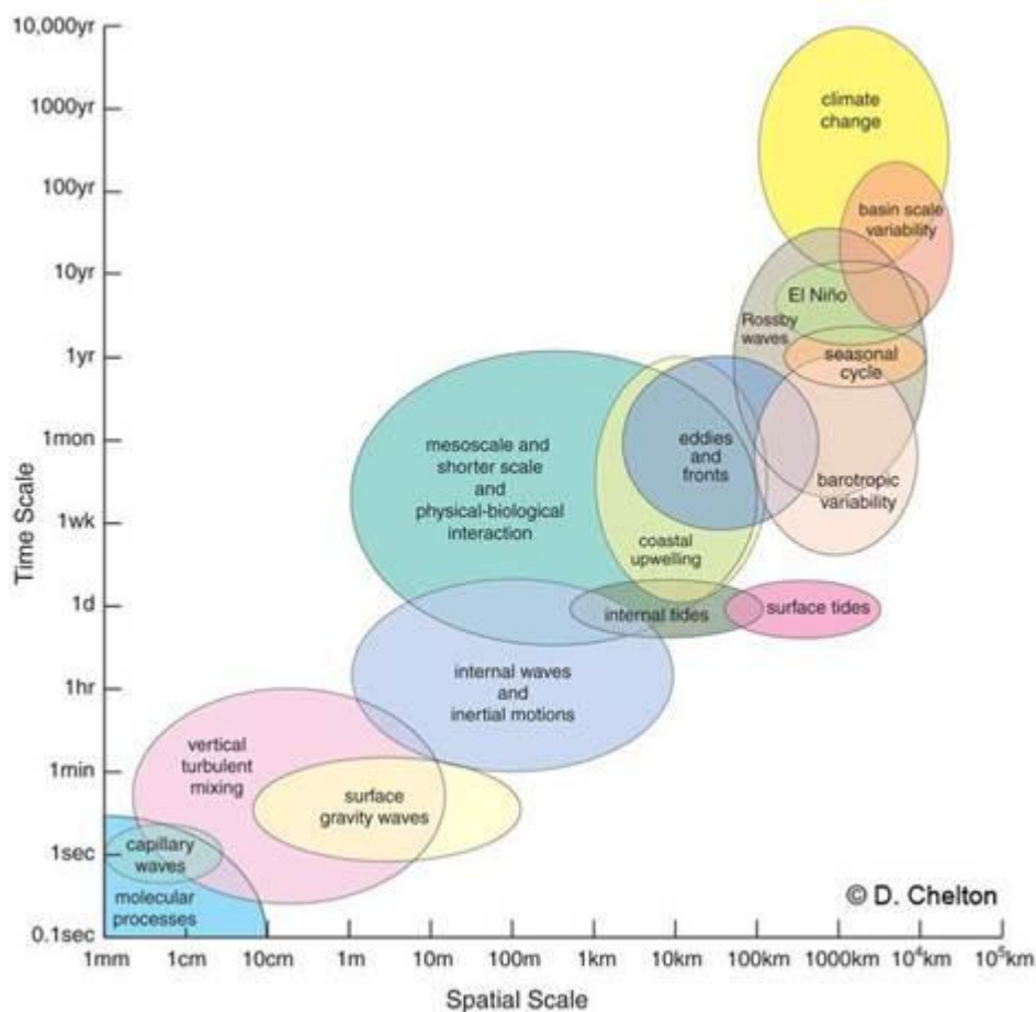
Figure 5.2.1. Time scales of ocean processes
