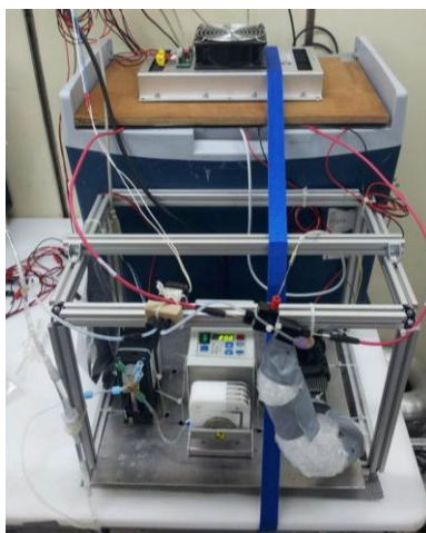
Figure 4.4.7. HZG spectrophotometric pH-sensor on a test bench.
