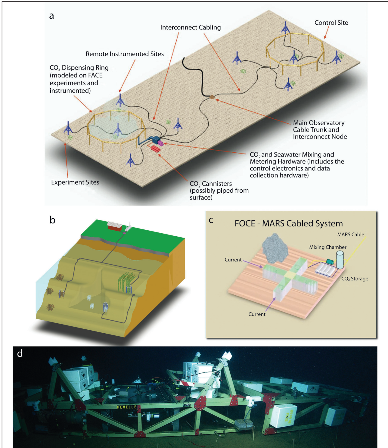
Figure 8.3 Free Ocean CO 2 Enrichment (FOCE) concepts and prototype. a. FOCE concept drawing with design analogous to FACE (Free Air CO 2 Enrichment) designs with coarse CO 2 plumbing and upstream CO 2 injection. b. FOCE concept for nearshore systems with shore-based supply and control stations leading to offshore FOCE plumbing frames. c. FOCE prototype design for connection to the Monterey Accelerated Research System (MARS) submarine cabled observatory. This system uses a flume design allowing flow into a control volume along 2 axes. d. Photograph of FOCE prototype at 900 m depth off Central California, attached for testing to the MARS cable system. Flow is along 1 axis, with a central control volume (behind “Revelle” label), flotation blocks (white blocks) for deployment/recovery, and a mixing zone in the upstream and downstream ends. (W. Kirkwood & MBARI).
