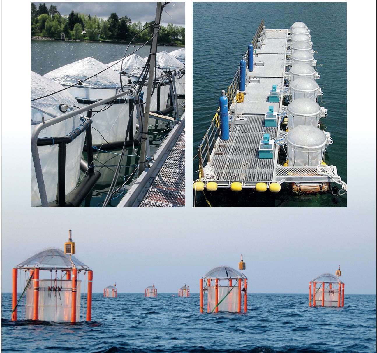
Figure 6.1 Mesocosm studies in ocean acidification research - upper left : PeECE III study in the Espegrend Marine Biological Station, Bergen, Norway (Riebesell et al. , 2008a); upper right : mesocosm facility at Jangmok on the southern coast of Korea (Kim et al. , 2008); lower panel : free-floating mesocosms deployed in the Baltic Sea (Riebesell et al. , unpubl.).
