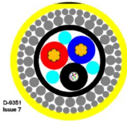
Figure 17. Section of the fiber and power cable.
