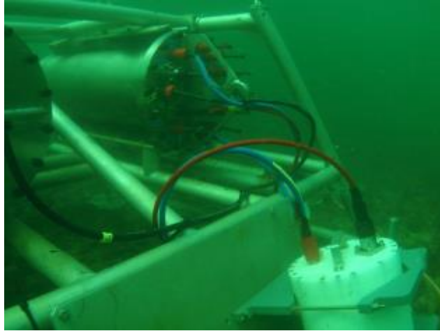
Figure 25. Connection between UNH node and instruments.
