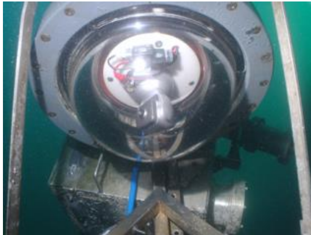
Figure 26. UNS underwater webcam system used to monitor the area.
