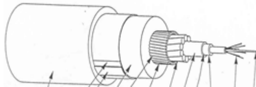
Figure 10. The OBSEA hybrid cable, deployed from land to the subsea node.
