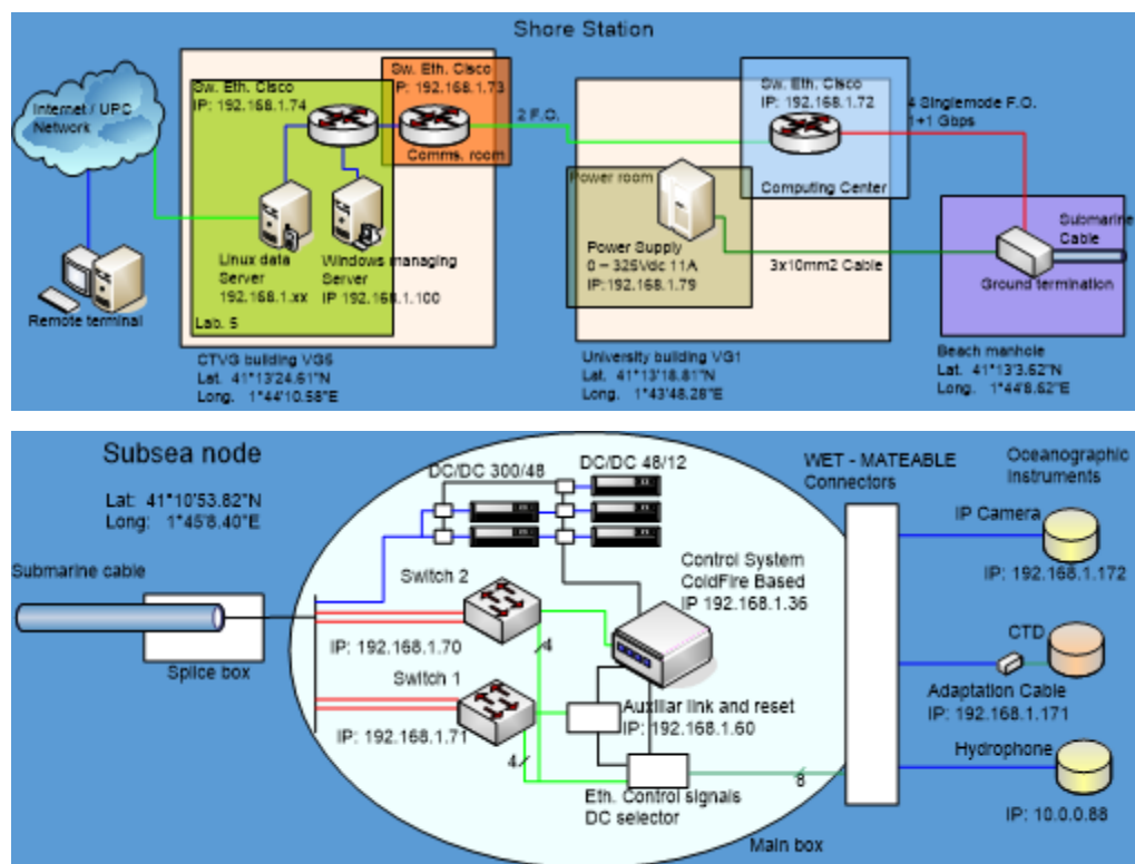
Figure 11. The OBSEA network.
