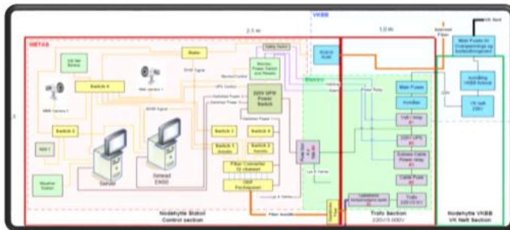
Figure 23. An overview of the LoVe Network.
