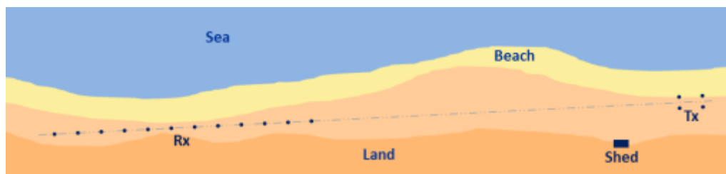
Figure 1. Typical setup of a phased array HF-radar system.
