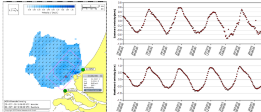
Figure 4. Surface current map from 26.October 2015 at 9:00 UTC resulting from the HF-radar network at the Hook of Holland, southern North Sea (left panel). The upper and lower panels on the right show the eastward and northward components of the surface currents over a 56 h period at the location marked by the red dot in the map on the left.
