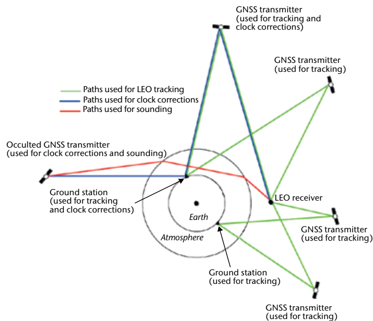
Figure 3.8. The overall system for radio occultation
