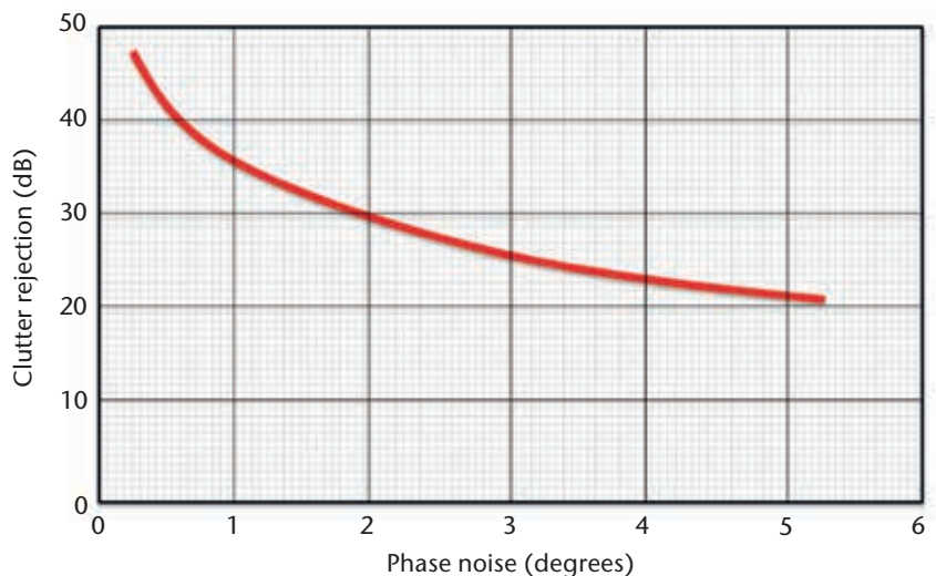
Figure 7.15. Coherency (phase noise) is a measure of the quality of a Doppler radar and is directly related to the ability to remove ground clutter and retrieve second-trip echoes using phase coding techniques.
