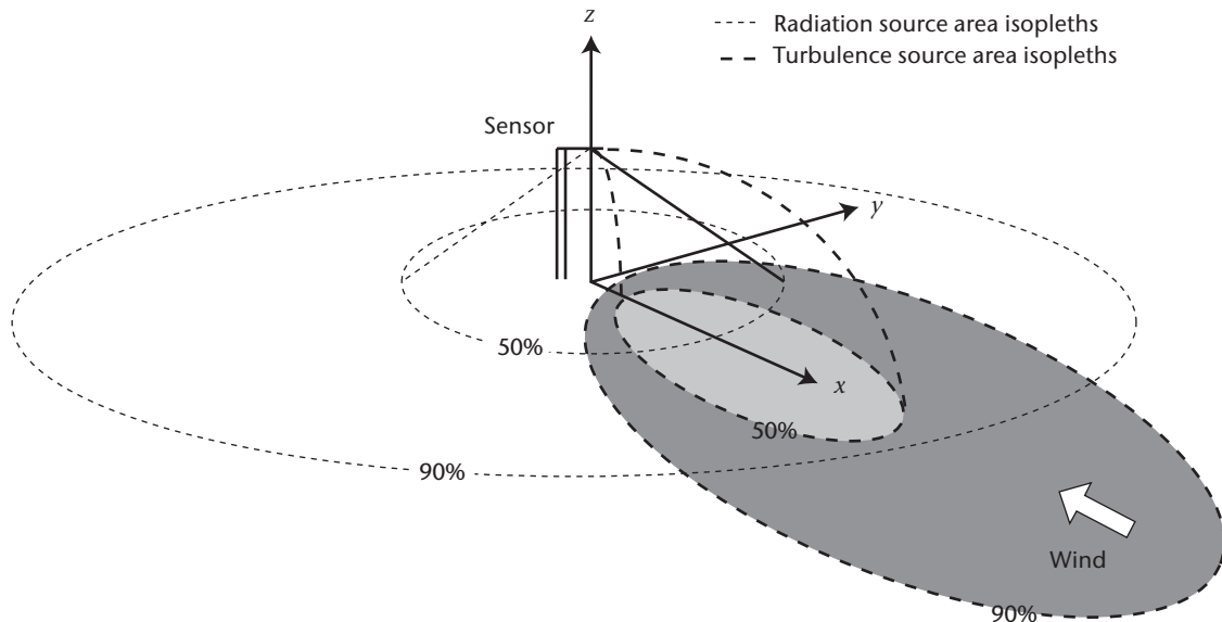
Figure 9.2. Conceptual representation of source areas contributing to sensors for radiation and turbulent fluxes of concentrations. If the sensor is a radiometer 50% or 90% of the flux originates from the area inside the perspective circle. If the sensor is responding to a property of turbulent transport, 50% or 90% of the signal comes from the area inside the respective ellipses. These are dynamic in the sense that they are oriented into the wind and hence move with wind direction and stability.
