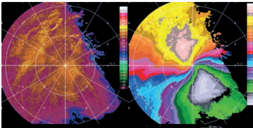
Figure 7.11. This figure illustrates the necessity and ability of a C band radar to extend the velocity out to at least 48 m s^{-1} . This is a case of a hurricane/extratropical transition passage and velocities are near 48 m s^{-1} . In this situation, the assumptions of the dual-PRF technique (the two measured estimates at different PRFs are from the same radial velocity) are satisfied and the result has little noise (right image, compare with Figure 7.20).
