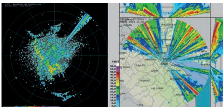
Figure 7.19. The image on the left demonstrates the type of expected interference from a Radio Local Area Network located 6.4 km away at 0.42° elevation angle. The image on the right is from an operational weather radar, courtesy of Claudia Competella of the Servicio Meteorológico Nacional (Argentina).
