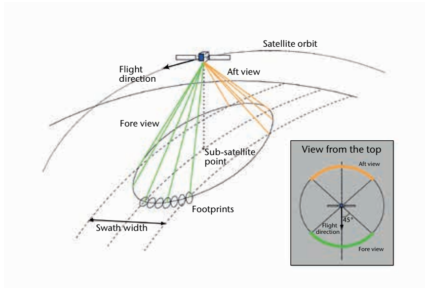
Figure 3.3. Geometry of conical scanning
