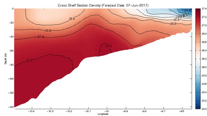
Figure 39. Model simulated (a) temperature ( ^{\circ}\text{C} ), (b) salinity and (c) density at ( \text{kg}\cdot\text{m}^{-3} ) along a southwest – northeast transect from 10^{\circ} 30' \text{ W} (0 km) on the continental shelf to inner Bantry Bay (70+ Km). This is one example of a number of transects where physical conditions are simulated, extracted and plotted on a daily operational basis to present local oceanographic phenomenon e.g. upwelling events in the local area of interest.
