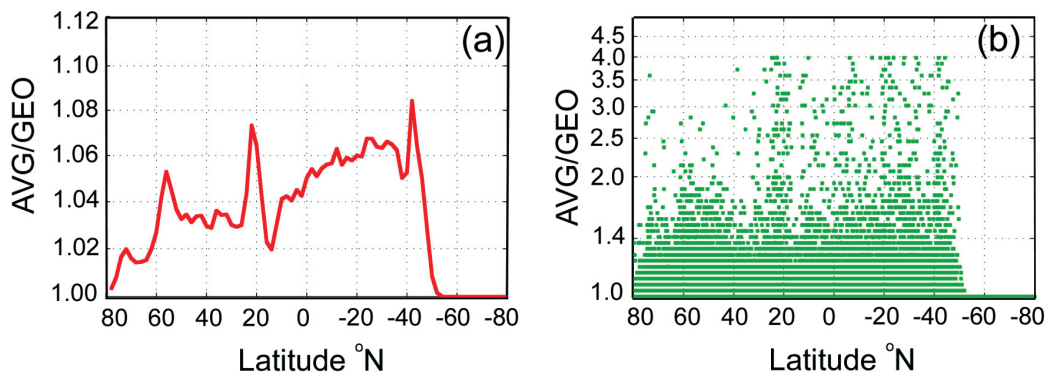
Figure 3.9 AVG/GEO ratios of monthly mean chlorophyll concentration. (a) Zonal average and (b) plots of each 0.25-degree grid.
