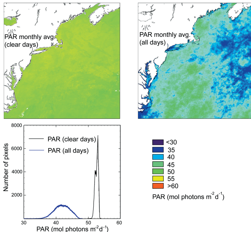
Figure 5.2 Monthly average PAR (units mol quanta \text{m}^{-2} \text{d}^{-1} ) used as input to derive \text{PP}_m^* (left) and \text{PP}_m (right). The image on the left shows the average of all clear-sky PAR values used in deriving \text{PP}_d .
