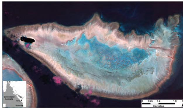
Figure 9.10 High-resolution Quickbird-2 satellite image acquired on 22 February 2004 showing coral-bleaching off Heron Island, Capricorn Bunker Group, Southern Great Barrier Reef, Australia. Image provided by Stuart Phinn and Chris Roelfsema, Center for Remote Sensing and Spatial Information Science, University of Queensland (Copyright DigitalGlobe).
