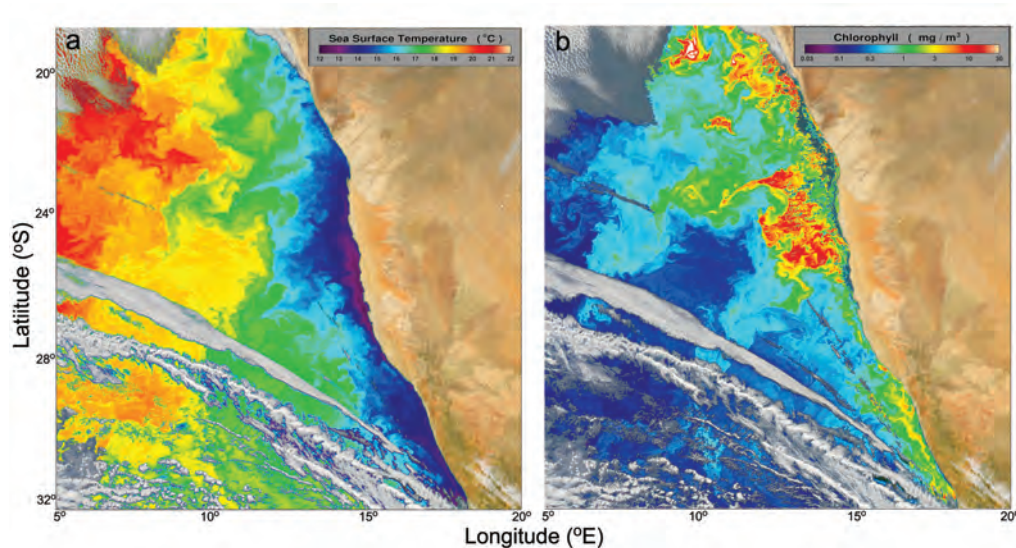
Figure 9.11 MODIS-Aqua SST and chlorophyll images from 17 June 2007 showing a) upwelling of cold (shown in blue) nutrient-rich water off the coast of Namibia, southern Africa and b) the associated high chlorophyll concentrations (shown in red) from a dense phytoplankton bloom (Credit: Ocean Biology Processing Group, NASA/GSFC).
