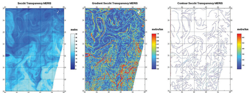
Figure 2.8 Example of structure detection for a MERIS scene (9 April 2003 in Indian Ocean). From left to right: transparency map, gradient map, contour map. Spatial resolution is 1 km. Illustration of a service delivery to the French “Service Hydrographique de la Marine” (image courtesy of ACRI-ST).
