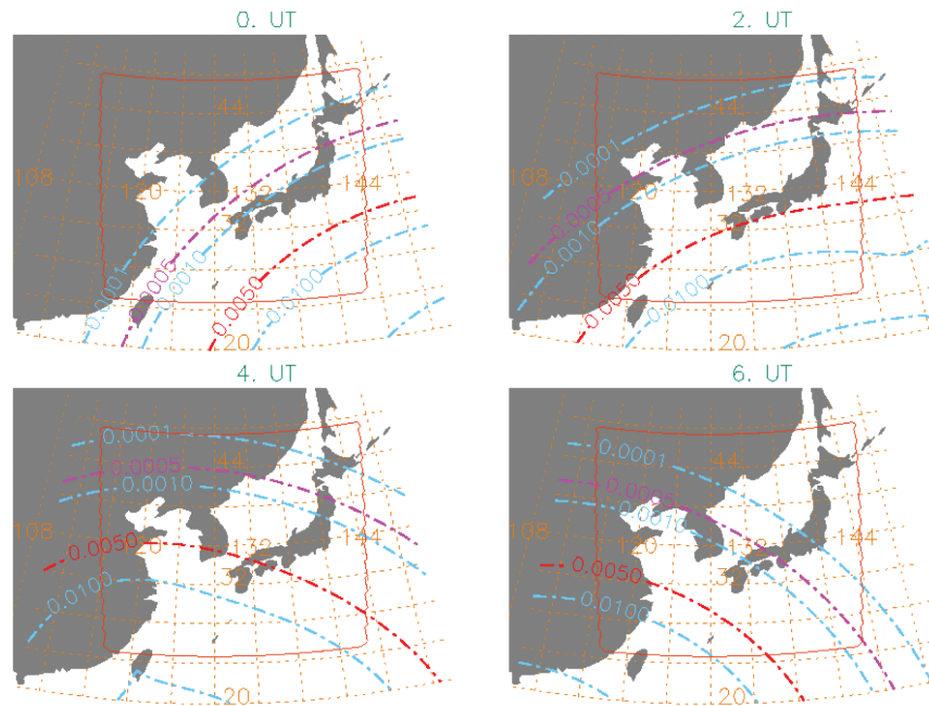
Simulated sunglint reflectance for C... the sunglint migrates maximally to the... of 10m/s. Image courtesy of P.Y. De...
