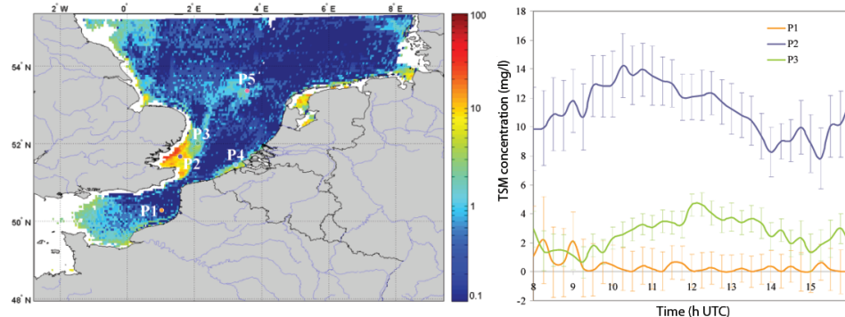
Left: TSM ( \text{mg l}^{-1} ) concentration maps. High frequency variability of TSM is observed. The error bars denote the estimated uncertainty on the TSM concentration introduced by the atmospheric correction assumptions.
