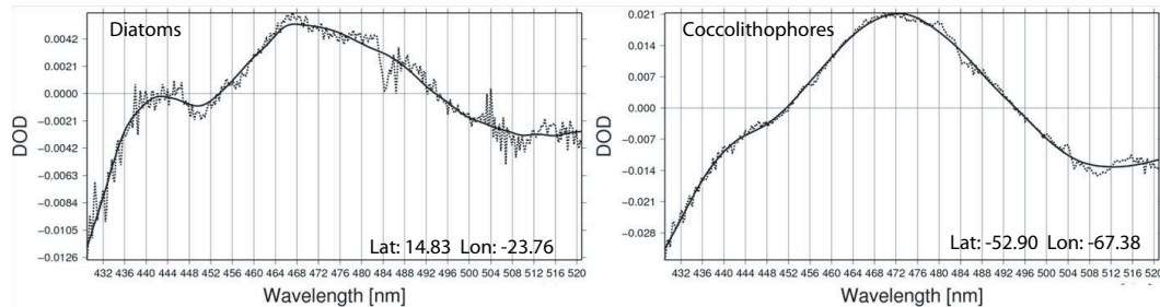
Figure 5.4 Spectral differential optical depth of SCIAMACHY data (dotted line) and the corresponding fit (straight line) for diatoms (left) and coccolithophores (right) using the specific differential absorption coefficients of each type scaled to match the observations according to the PhytoDOAS method described in Sadeghi et al. (2012a).
