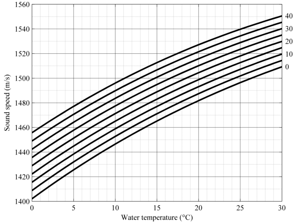
Figure 2.6. Variation of sound speed with water temperature, t_w ( ^{\circ}\text{C} ), and salinity, s_w (psu, as indicated on the right axis). Calculated from the nine-term equation in (Mackenzie, 1981).
