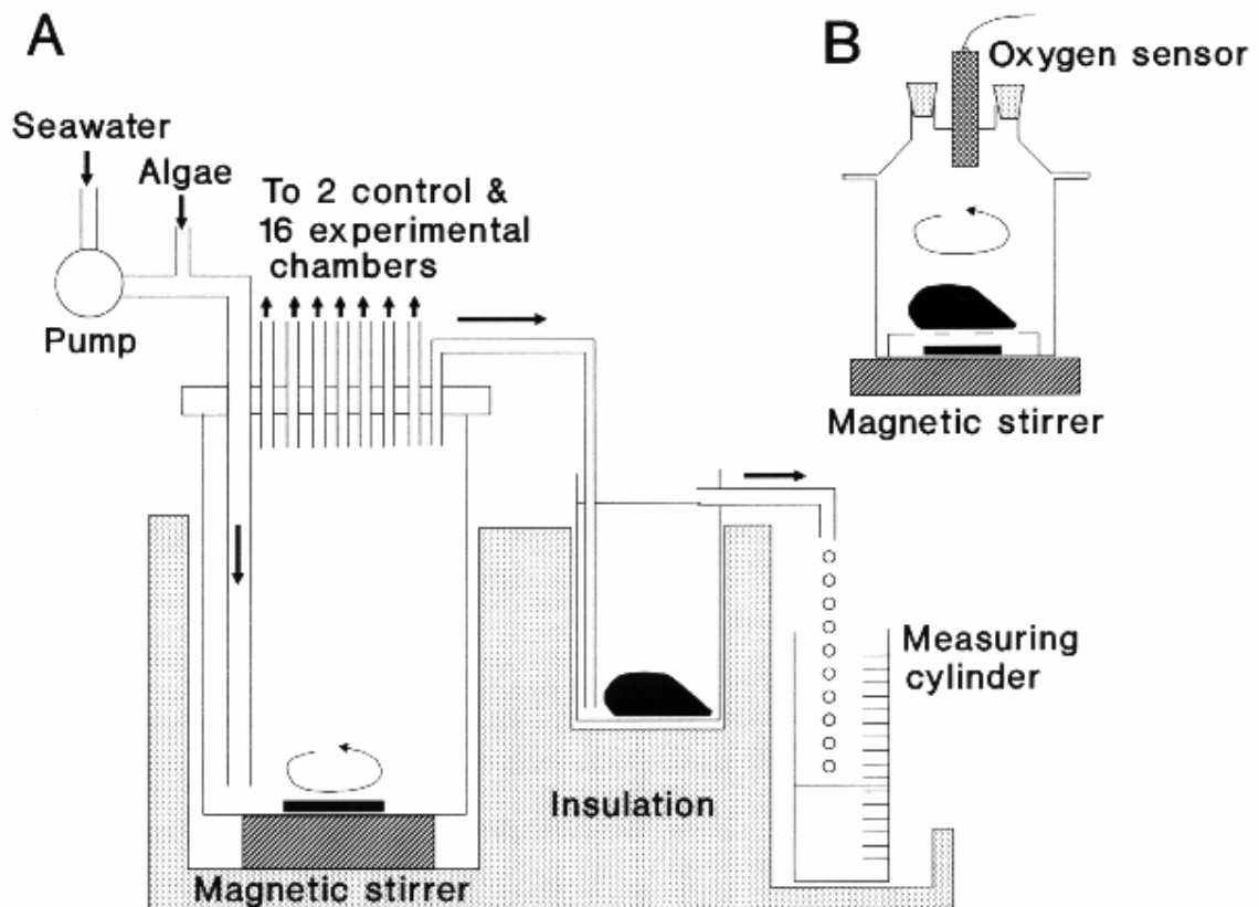
Figure 1A. Flow-through apparatus for maintaining and feeding of mussels. Figure 1B. Glass respirometer for measurement of oxygen consumption.
