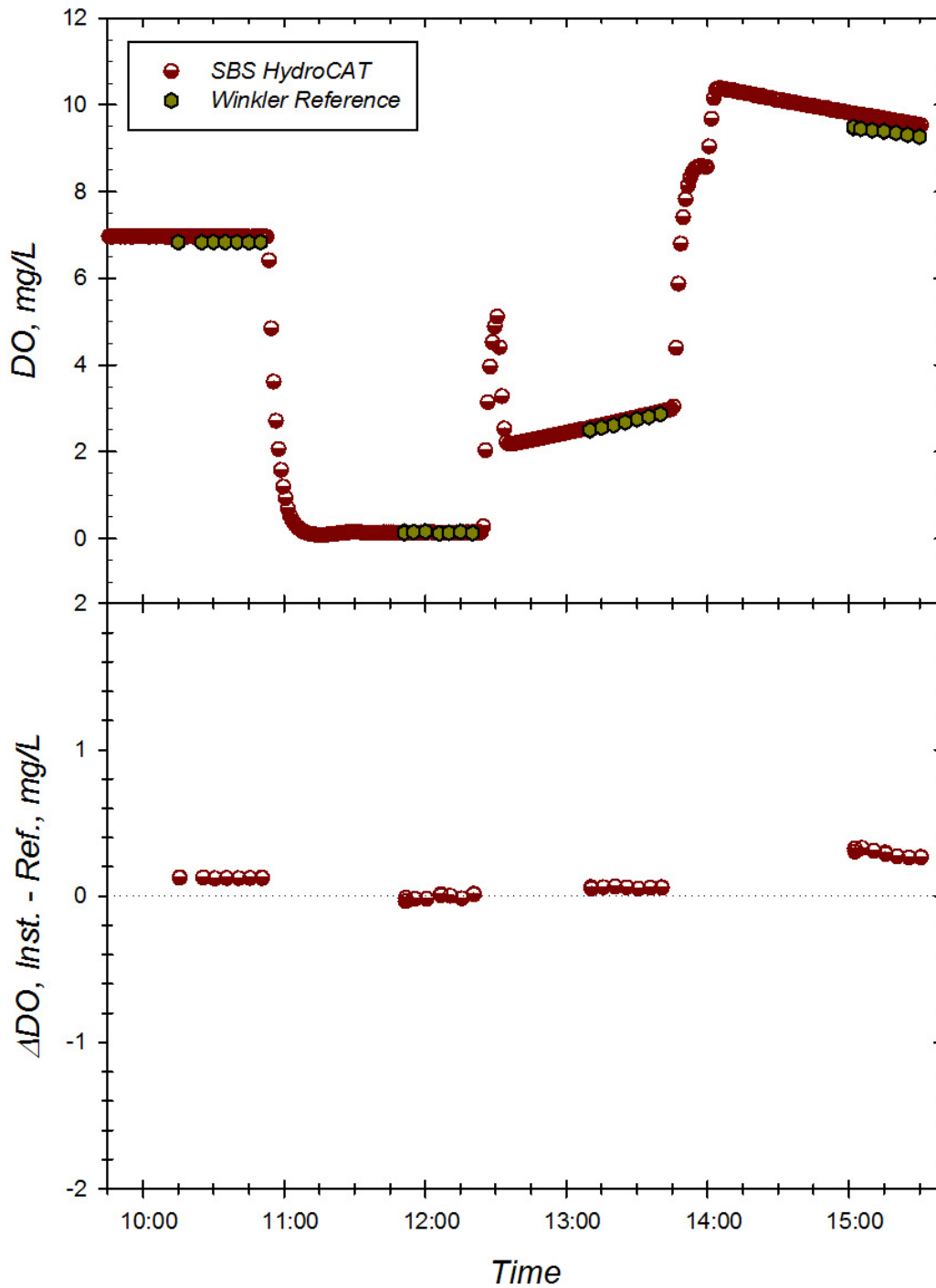
Figure H. Response of the SBS HydroCAT (SN 03710297) to changing dissolved oxygen concentrations at 30.5 °C and S=9.28. Top Panel: Time series of instrument readings and Winkler reference samples drawn at level of sensor foil in well-mixed test tanks. Bottom Panel: Corresponding offset between instrument reading and Winkler DO reference sample during exposure trial. Dotted line represents zero offset from reference.
