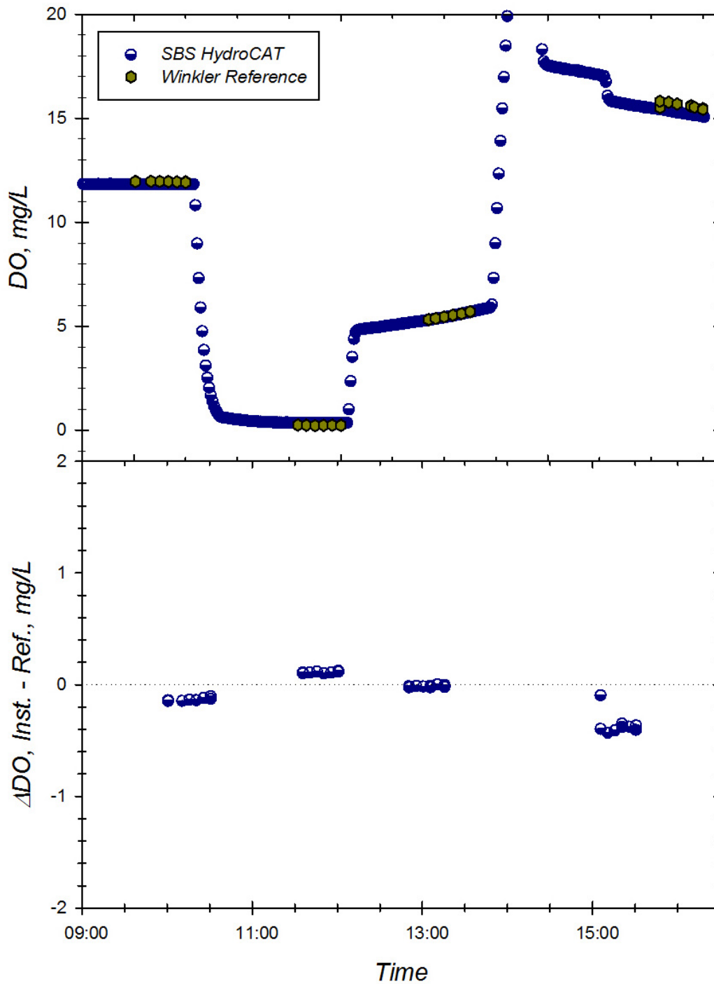
Figure E. Response of the SBS HydroCAT (SN 03710297) to changing dissolved oxygen concentrations at 5.3 °C and S=8.98. Top Panel: Time series of instrument readings and Winkler reference samples drawn at level of sensor foil in well-mixed test tanks. Bottom Panel: Corresponding offset between instrument reading and Winkler DO reference sample during exposure trial. Dotted line represents zero offset from reference.
