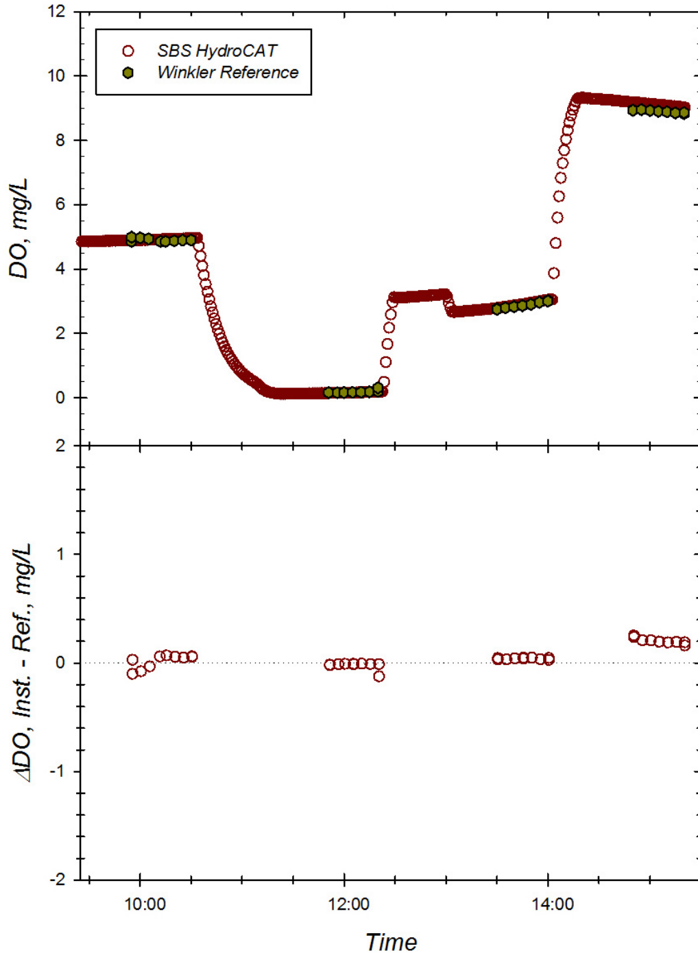
Figure G. Response of the SBS HydroCAT (SN 03710297) to changing dissolved oxygen concentrations at 30.2 °C and S=0.00. Top Panel: Time series of instrument readings and Winkler reference samples drawn at level of sensor foil in well-mixed test tanks. Bottom Panel: Corresponding offset between instrument reading and Winkler DO reference sample during exposure trial. Dotted line represents zero offset from reference.
