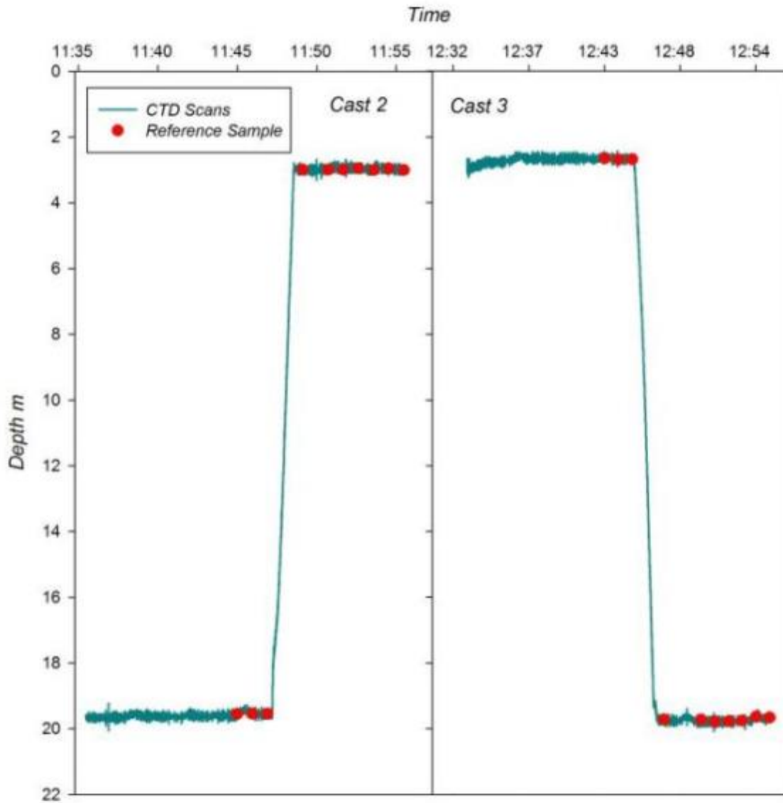
Figure 11. Time series of the rosette profiling and Niskin bottle sampling for the two profiling trials in Muskegon Lake.
