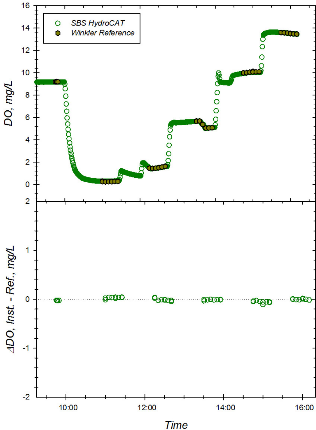
Figure A. Response of the SBS HydroCAT (SN 03710297) to changing dissolved oxygen concentrations at 15.4 °C and S=0.00. Top Panel: Time series of instrument readings and Winkler reference samples drawn at level of sensor foil in well-mixed test tanks. Bottom Panel: Corresponding offset between instrument reading and Winkler DO reference sample during exposure trial. Dotted line represents zero offset from reference.
