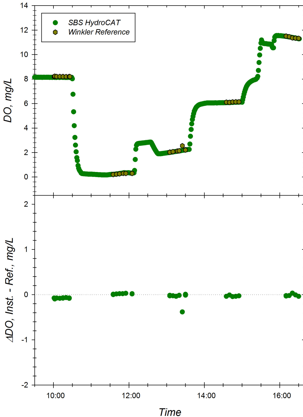
Figure C. Response of the SBS HydroCAT (SN 03710297) to changing dissolved oxygen concentrations at 15.4 °C and S=34.20. Top Panel: Time series of instrument readings and Winkler reference samples drawn at level of sensor foil in well-mixed test tanks. Bottom Panel: Corresponding offset between instrument reading and Winkler DO reference sample during exposure trial. Dotted line represents zero offset from reference.
