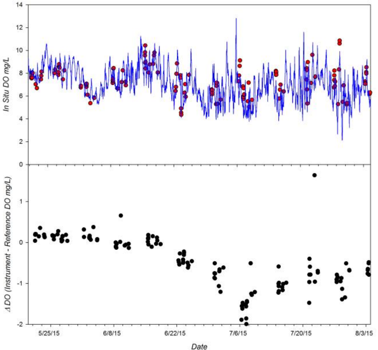
Figure 5. Time series of DO measured by the SBS HydroCAT during the 12 week CBL field trial. Top Panel: Continuous DO recordings from instrument (blue line) and DO of adjacent grab samples determined by Winkler titration (red circles). Bottom Panel: Difference in measured DO relative to reference samples (Instrument DO mg/L – Reference DO mg/L) observed during deployment.
