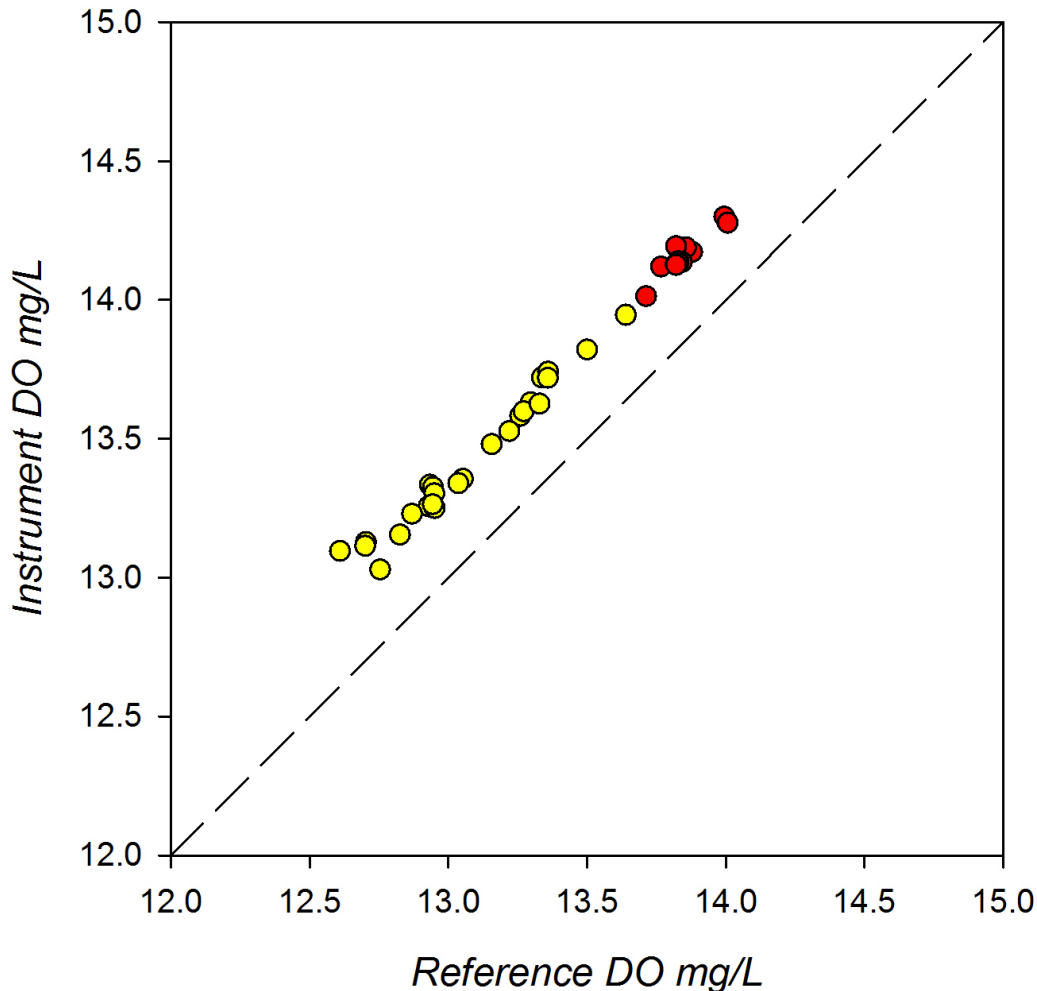
Figure 3. MTU GLRI field response plot for the first month of deployment of SBS instrument compared to reference DO samples. The plotted line represents a 1:1 correspondence. . (Yellow circles denote adjusted reference values).
