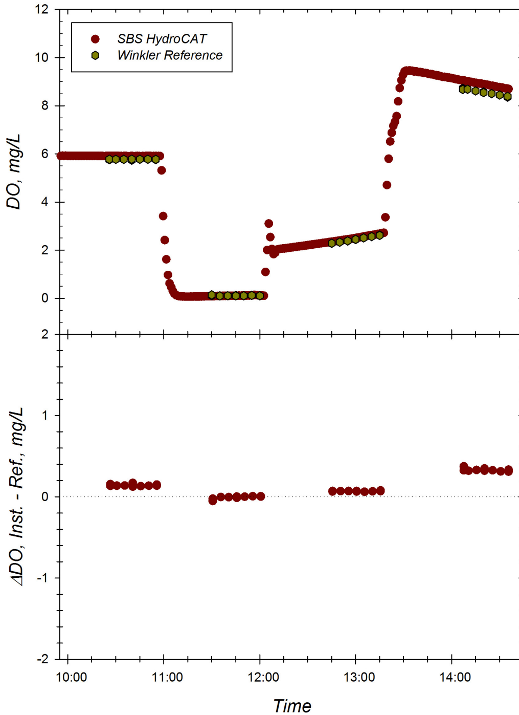
Figure I. Response of the SBS HydroCAT (SN 03710297) to changing dissolved oxygen concentrations at 30.6 °C and S=34.43. Top Panel: Time series of instrument readings and Winkler reference samples drawn at level of sensor foil in well-mixed test tanks. Bottom Panel: Corresponding offset between instrument reading and Winkler DO reference sample during exposure trial. Dotted line represents zero offset from reference
