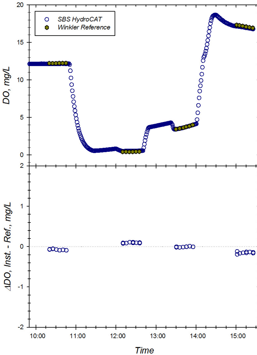
Figure D. Response of the SBS HydroCAT (SN 03710297) to changing dissolved oxygen concentrations at 5.4 °C and S=0.00. Top Panel: Time series of instrument readings and Winkler reference samples drawn at level of sensor foil in well-mixed test tanks. Bottom Panel: Corresponding offset between instrument reading and Winkler DO reference sample during exposure trial. Dotted line represents zero offset from reference.
