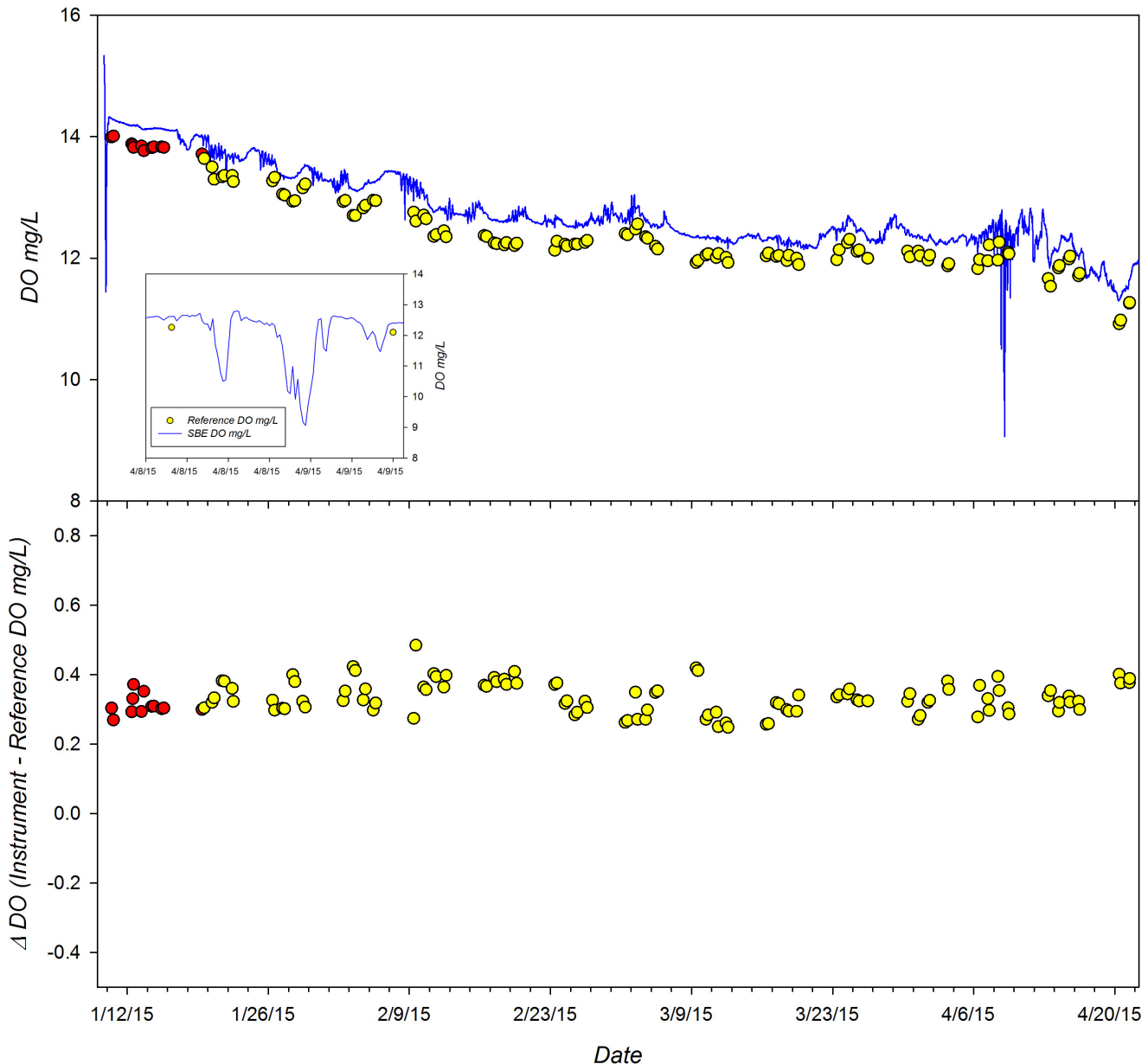
Figure 2. Time series of DO measured detected by SBS HydroCAT deployed during the 15 week Great Lakes field trial. Top Panel: Continuous DO recordings from instrument (blue line) and DO of adjacent grab samples determined by Winkler titration (red circles; yellow circles represent adjusted reference values). Bottom Panel: Difference in measured DO relative to reference samples (Instrument DO mg/L – Ref DO mg/L) observed during deployment. Insert: Close up of excursion that occurred 4/8-4/9. No reference samples were collected during this time period.
