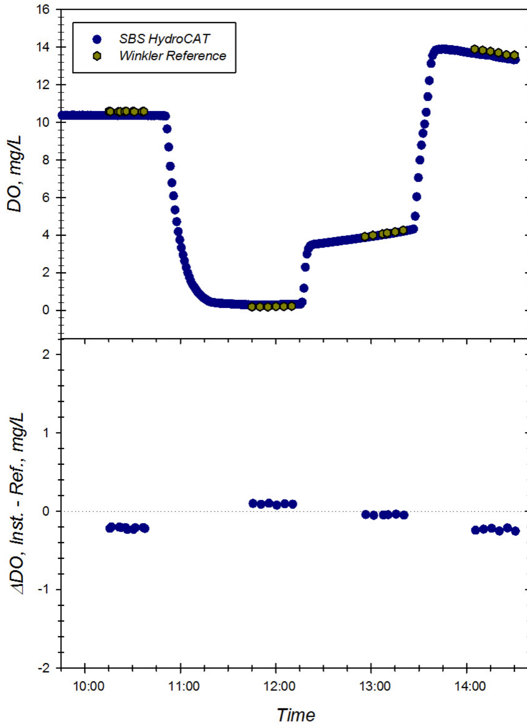
Figure F. Response of the SBS HydroCAT (SN 03710297) to changing dissolved oxygen concentrations at 5.2 °C and S=34.77. Top Panel: Time series of instrument readings and Winkler reference samples drawn at level of sensor foil in well-mixed test tanks. Bottom Panel: Corresponding offset between instrument reading and Winkler DO reference sample during exposure trial. Dotted line represents zero offset from reference.
