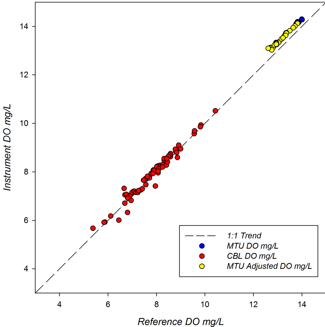
Figure 10. Global response plot for the SBS HydroCAT instruments observed during the three ACT field trials. Black dotted line represents a 1:1 correspondence.
