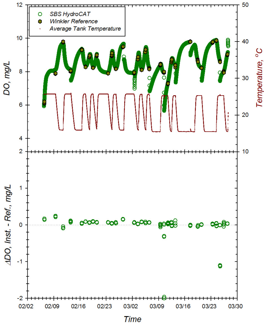
Figure K. Long-term stability and thermal stress challenge of the SBS HydroCAT (SN 03710297). Instrument was maintained in well circulated tank and oxygen content manipulated by alternately varying water temperature set point between 15 and 25 °C several times per week of deployment. Top Panel: Time series of the instrument readings at 15min intervals with discrete values for Winkler assay of grab samples taken at sensor level. Bottom Panel: Offset in paired DO readings of and Winkler grab samples.
