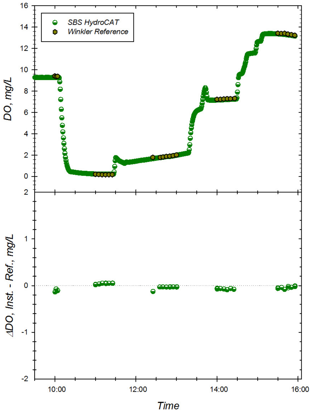
Figure B. Response of the SBS HydroCAT (SN 03710297) to changing dissolved oxygen concentrations at 15.4 °C and S=8.82. Top Panel: Time series of instrument readings and Winkler reference samples drawn at level of sensor foil in well-mixed test tanks. Bottom Panel: Corresponding offset between instrument reading and Winkler DO reference sample during exposure trial. Dotted line represents zero offset from reference.
