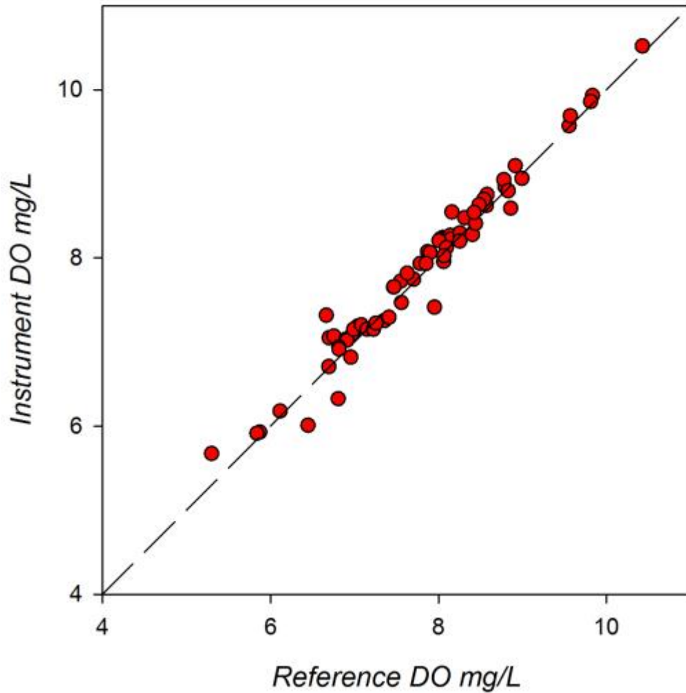
Figure 6. CBL field response plot for SBS HydroCAT compared to reference DO samples. The plotted line represents a 1:1 correspondence.
