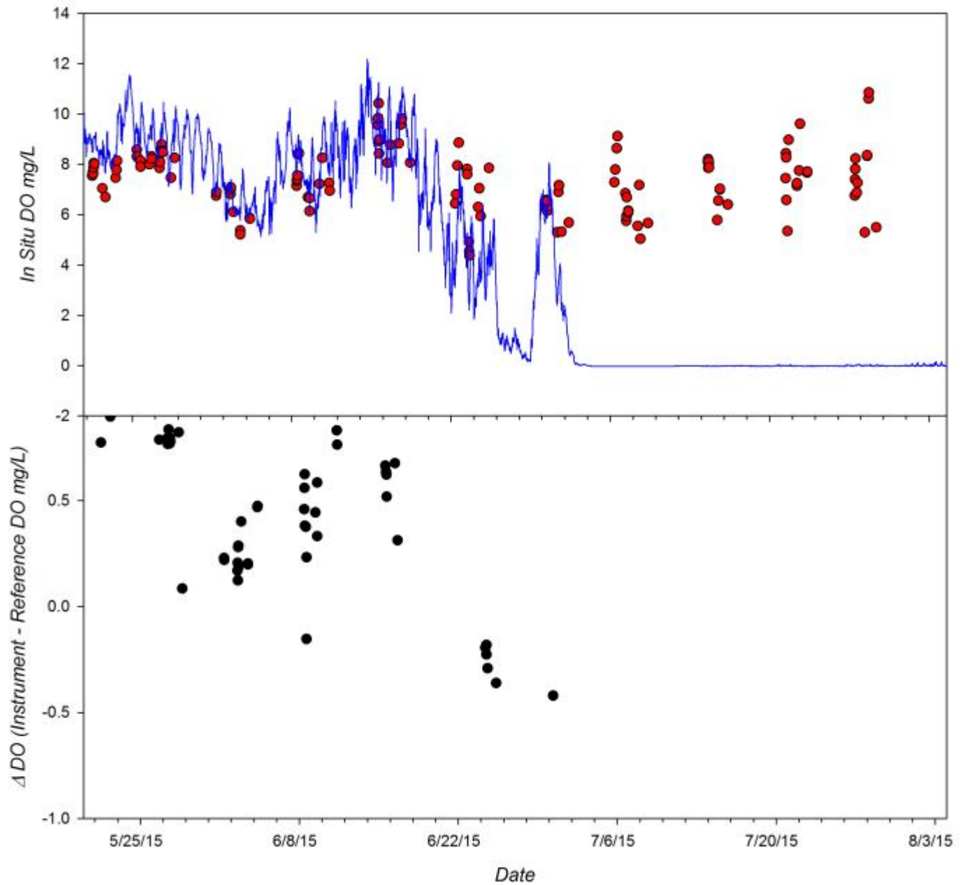
Figure 5. Time series of DO measured by the Troll during the 12 week CBL field trial. Top Panel: Continuous DO recordings from instrument (blue line) and DO of adjacent grab samples determined by Winkler titration (red circles). Bottom Panel: The difference in measured DO relative to reference samples (Instrument DO mg/L – Ref DO mg/L) observed during deployment.
