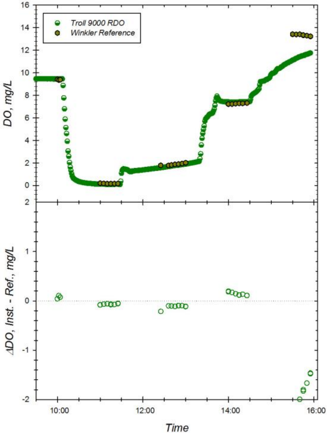
Figure B. Response of Troll 9000 with Optical DO (sn 51530) to changing dissolved oxygen concentrations at 15.4°C and S=8.82. Top Panel: Time series of instrument readings and Winkler reference samples drawn at level of sensor foil in well-mixed test tanks. Bottom Panel: Corresponding offset between instrument reading and Winkler DO reference sample during exposure trial. Dotted line represents zero offset from reference.
