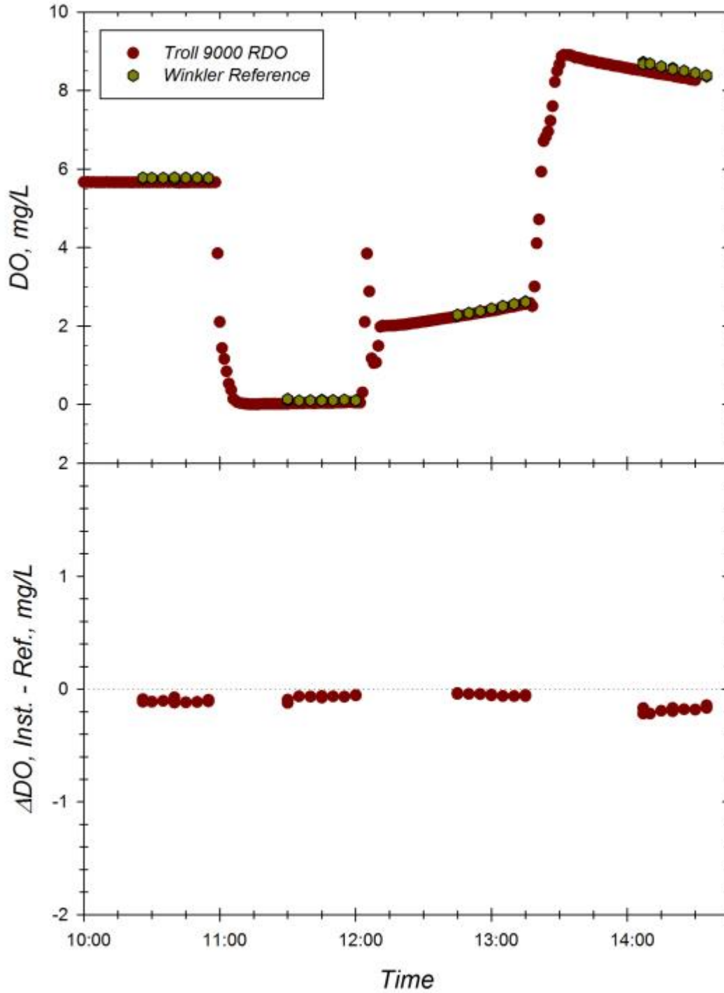
Figure I. Response of Troll 9000 with Optical DO (sn 51530) to changing dissolved oxygen concentrations at 30.6 °C and S=34.43. Top Panel: Time series of instrument readings and Winkler reference samples drawn at level of sensor foil in well-mixed test tanks. Bottom Panel: Corresponding offset between instrument reading and Winkler DO reference sample during exposure trial. Dotted line represents zero offset from reference.
