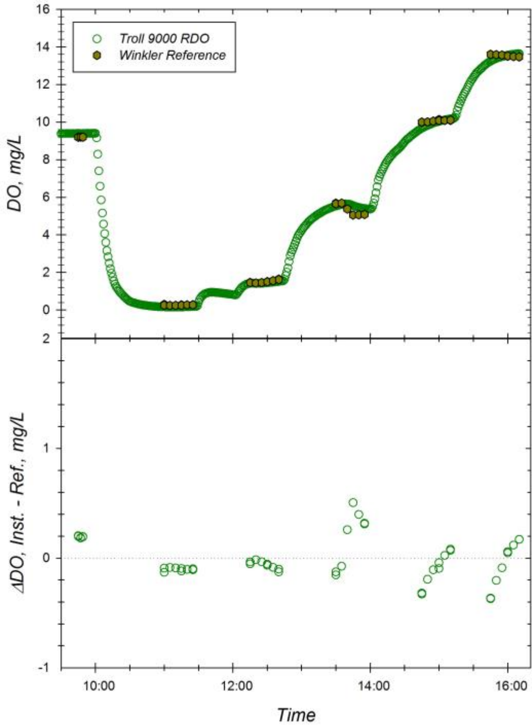
Figure A. Response of Troll 9000 with Optical DO (sn 51530) to changing dissolved oxygen concentrations at 15.4°C and S=0.00. Top Panel: Time series of instrument readings and Winkler reference samples drawn at level of sensor foil in well-mixed test tanks. Bottom Panel: Corresponding offset between instrument reading and Winkler DO reference sample during exposure trial. Dotted line represents zero offset from reference.
