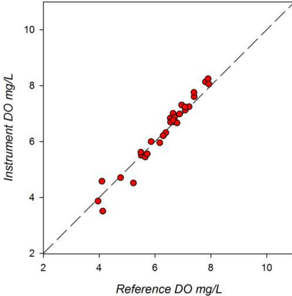
Figure 9. HIMB field response plot of Troll 9000 compared to reference DO samples determined by Winkler Titration. The plotted line represents a 1:1 correspondence.
