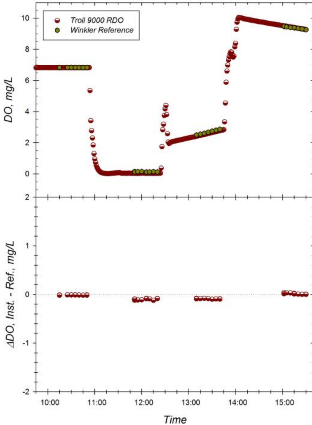
Figure H. Response of Troll 9000 with Optical DO (sn 51530) to changing dissolved oxygen concentrations at 30.5 °C and S=9.28. Top Panel: Time series of instrument readings and Winkler reference samples drawn at level of sensor foil in well-mixed test tanks. Bottom Panel: Corresponding offset between instrument reading and Winkler DO reference sample during exposure trial. Dotted line represents zero offset from reference.
