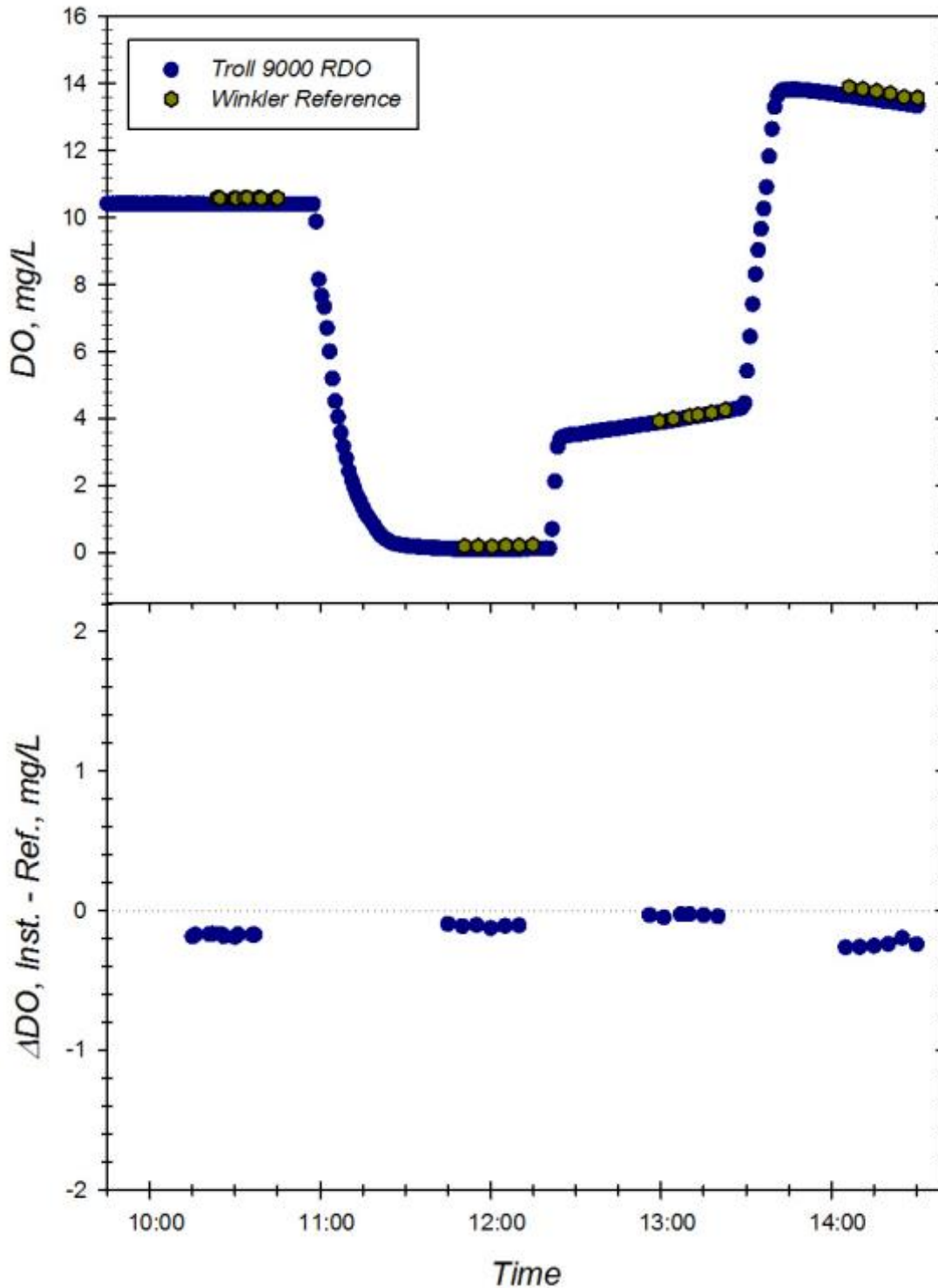
Figure F. Response of Troll 9000 with Optical DO (sn 51530) to changing dissolved oxygen concentrations at 5.2°C and S=34.77. Top Panel: Time series of instrument readings and Winkler reference samples drawn at level of sensor foil in well-mixed test tanks. Bottom Panel: Corresponding offset between instrument reading and Winkler DO reference sample during exposure trial. Dotted line represents zero offset from reference.
