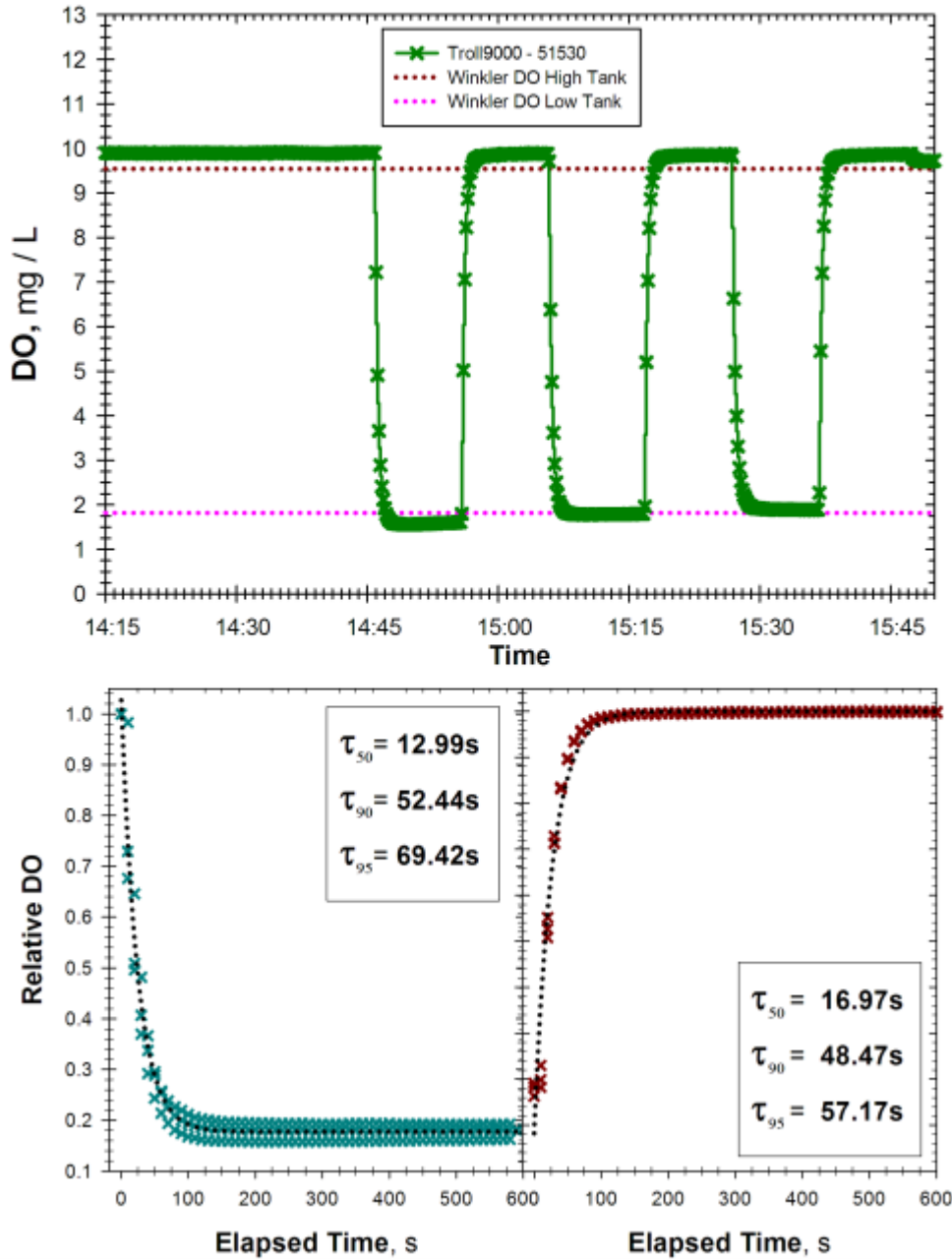
Figure L. Assessment of the sensor response time for the Troll 9000 with Optical DO (sn 51530). Top Panel: Time series of 10s reads of instruments during transfers between high and low DO buckets maintained adjacent in a common water bath equilibrated at 15°C. Indicated DO levels were maintained by airstone bubblers (high DO) or air+N 2 (low DO) and verified by Winkler assays. Bottom Panels: All high DO to low DO transitions were normalized to last reading before condition switch for the indicated time post transition (left). Data was fit with a 3 parameter exponential decay function: DO_{rel} = DO_{relMin} + ae^{-bt} and indicated \tau calculated from fit. Data for low DO to high DO transitions ( lower right ) were treated similarly but normalized to steady state value in subsequent high DO tank and subsequently fit with an analogous 3 parameter exponential rise function: DO_{rel} = DO_{relMin} + a(1 - e^{-bt}) with indicated \tau being directly calculated from fit.
