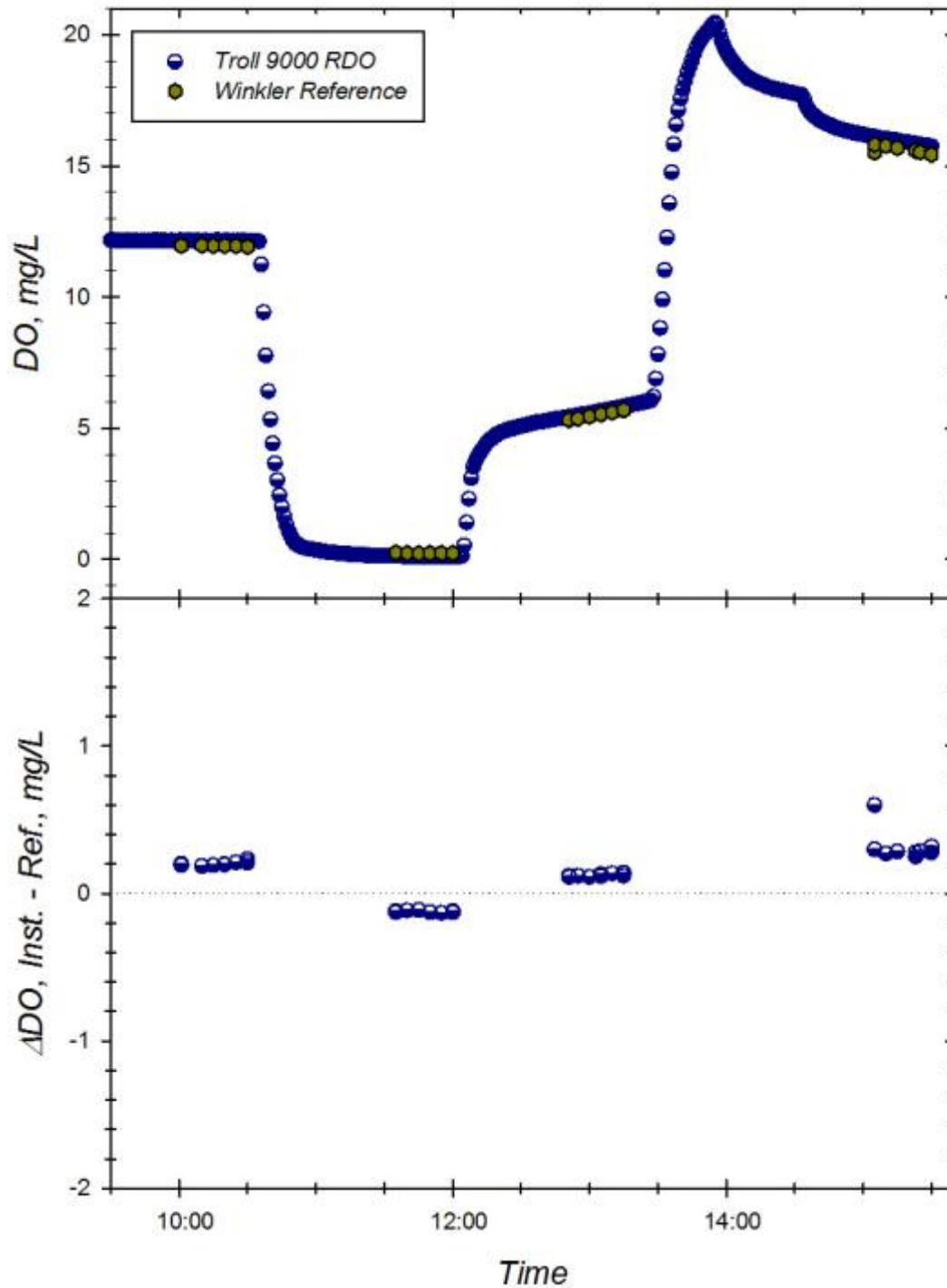
Figure E. Response of Troll 9000 with Optical DO (sn 51530) to changing dissolved oxygen concentrations at 5.3°C and S=8.98. Top Panel: Time series of instrument readings and Winkler reference samples drawn at level of sensor foil in well-mixed test tanks. Bottom Panel: Corresponding offset between instrument reading and Winkler DO reference sample during exposure trial. Dotted line represents zero offset from reference.
