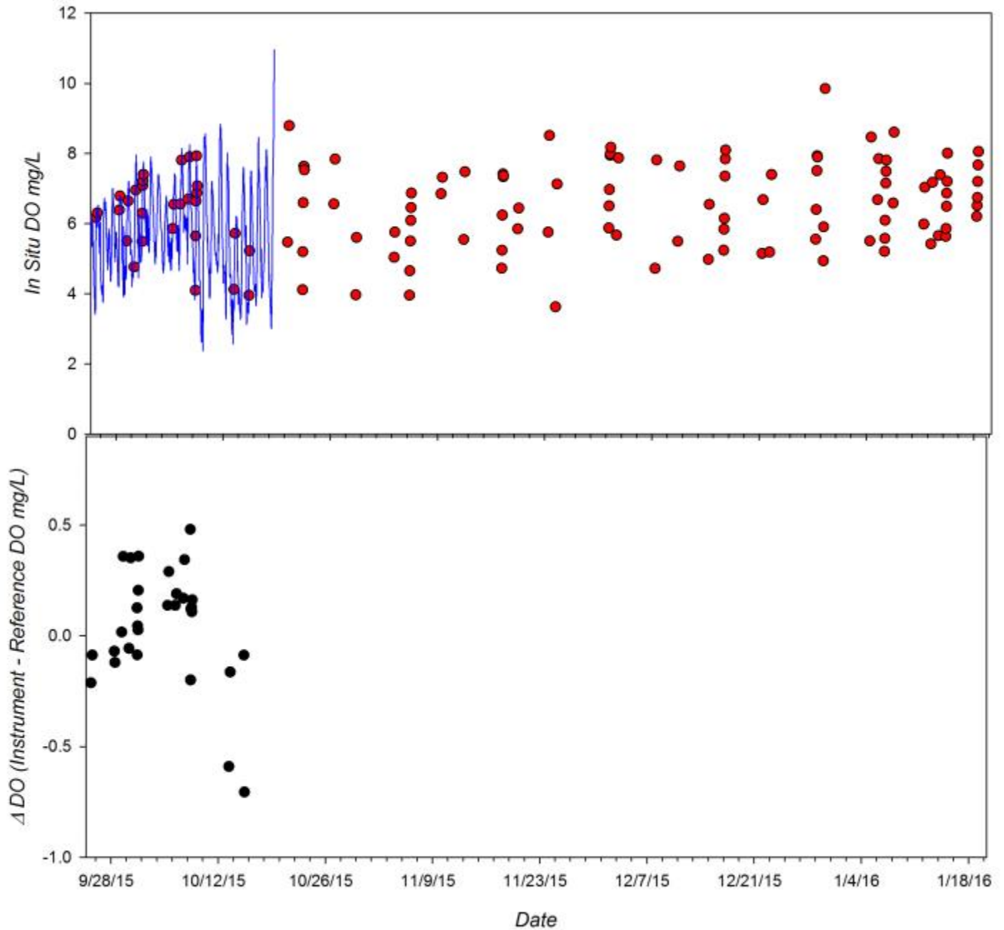
Figure 8. Top panel: Time series of DO measured by Troll 9000 deployed during the 18 week HIMB field trial. Continuous DO recordings from instrument (blue line) and DO of adjacent grab samples determined by Winkler Titrations (red circles.) Bottom Panel: Time series of the difference between the EXO2 and reference measurements for each matched pair (Instrument DO mg/L – Reference DO mg/L) in the range of \pm 2 mg/L DO (n=129 of a total possible 129 observations).
