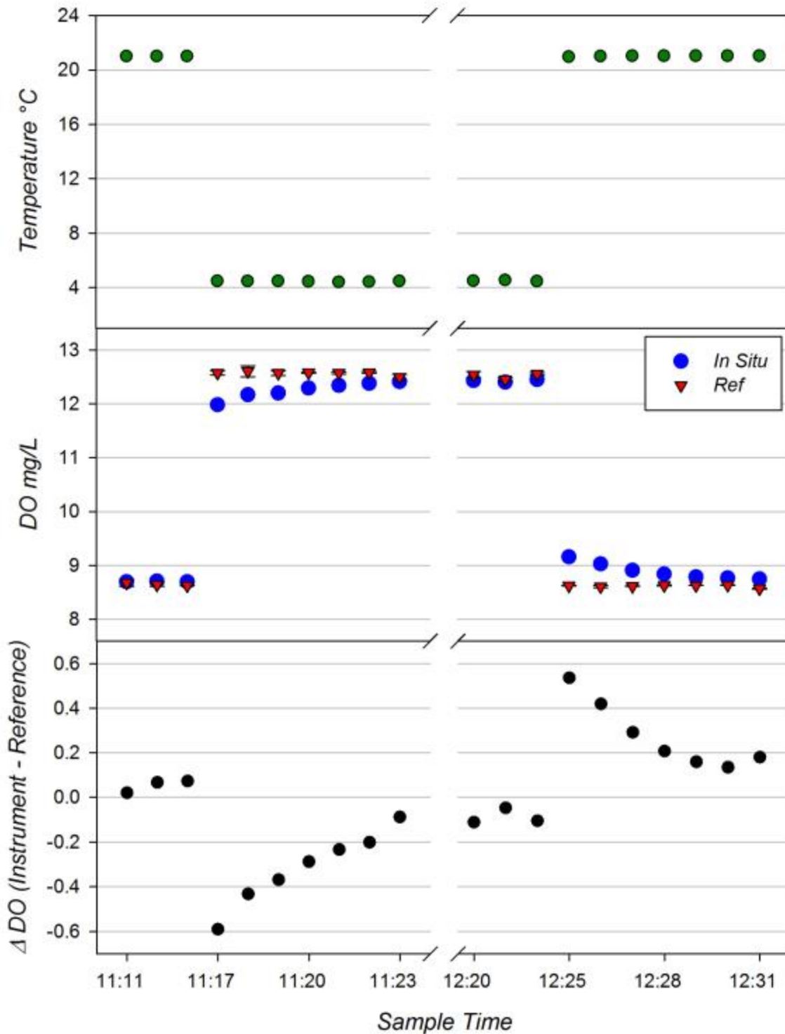
Figure 16. Results of the Troll 9000 for the Lake Michigan trials. Top panel: Troll 9000 temperature data at sample snap. Middle panel: DO recordings from instrument (blue dot) and DO of adjacent sample snaps determined by Winkler Titrations (red triangles.) Bottom panel: Time series of the difference between the Troll 9000 and reference measurements for each matched pair. Cast 1 and 2 are plotted on the same graph and separated by the axis break.
