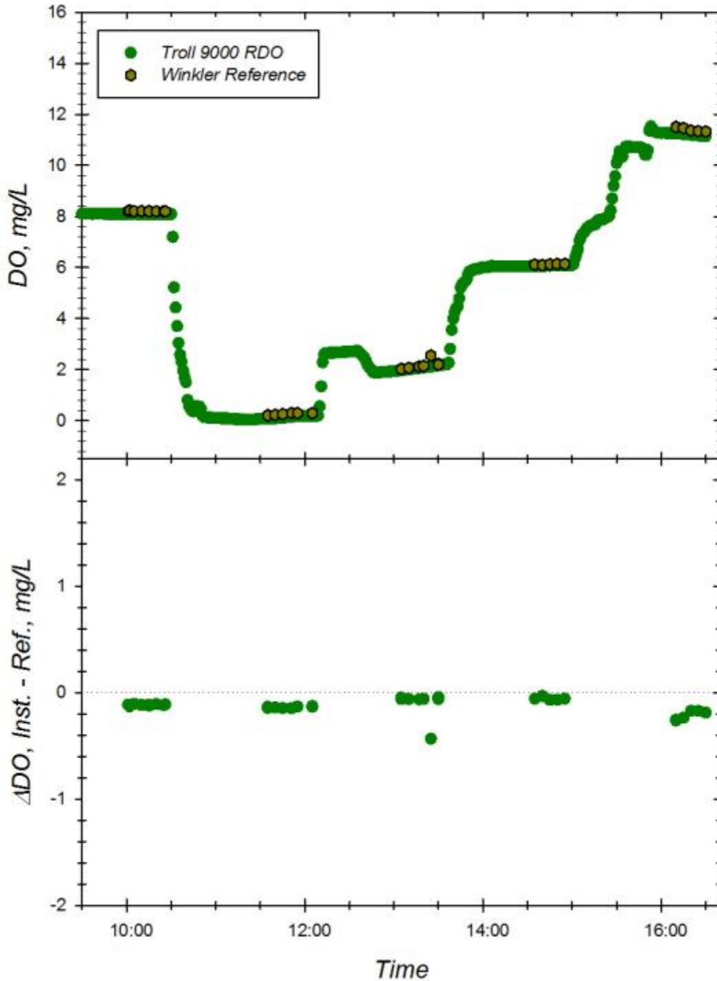
Figure C. Response of Troll 9000 with Optical DO (sn 51530) to changing dissolved oxygen concentrations at 15.4°C and S=34.20. Top Panel: Time series of instrument readings and Winkler reference samples drawn at level of sensor foil in well-mixed test tanks. Bottom Panel: Corresponding offset between instrument reading and Winkler DO reference sample during exposure trial. Dotted line represents zero offset from reference.
