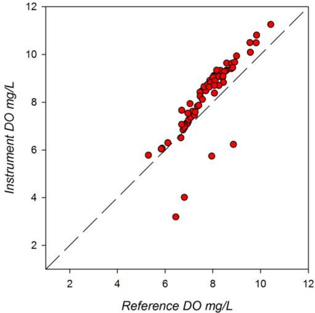
Figure 6. CBL field response plot for Troll compared to reference DO samples. The plotted line represents a 1:1 correspondence.
