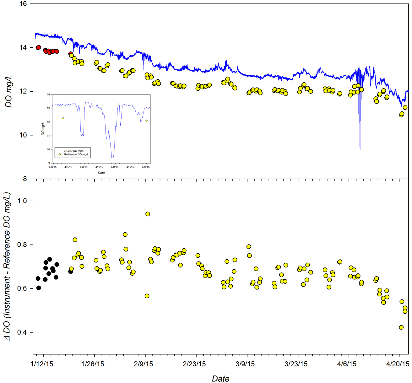
Figure 2. Time series of DO measured detected by Troll 9000 deployed during the 15 week Great Lakes field trial. Top Panel: Continuous DO recordings from instrument (blue line) and DO of adjacent grab samples determined by Winkler titration (red circles; yellow circles represent adjusted reference values). Bottom Panel: The difference in measured DO relative to reference samples ((Instrument DO mg/L – Ref DO mg/L) observed during deployment. Insert: Close up of excursion that occurred 4/8-4/9. No reference samples were collected during this time period.
