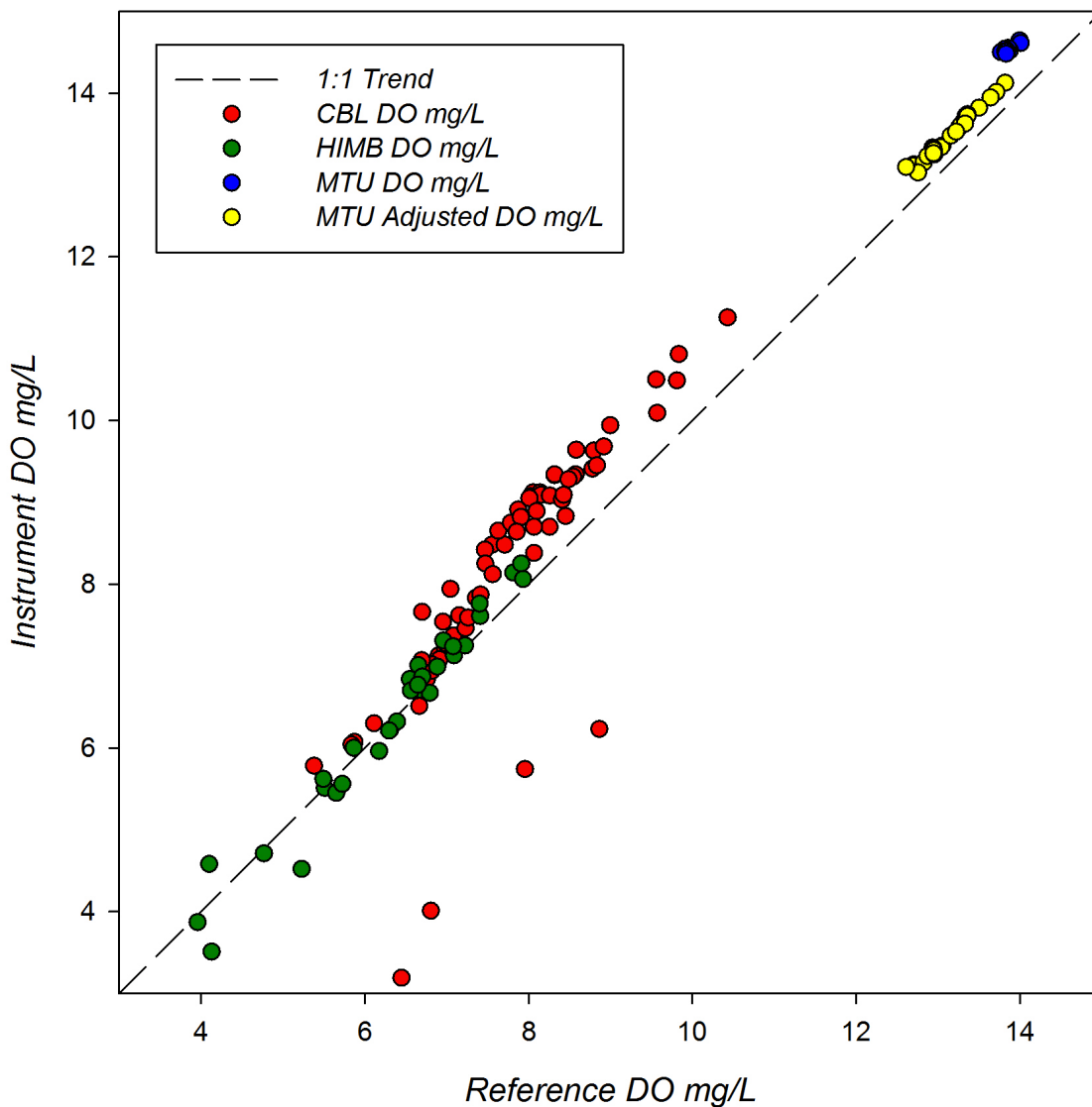
Figure 10. Global response plot for the Troll 9000 instruments observed during the three ACT field trials. Black dotted line represents a 1:1 correspondence.
