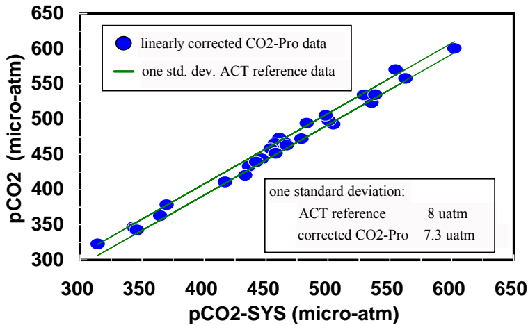
figure showing CO2-Pro data with calibration adjusted (blue) in relation to the one standard deviation estimated error for ACT wet chemical results.
