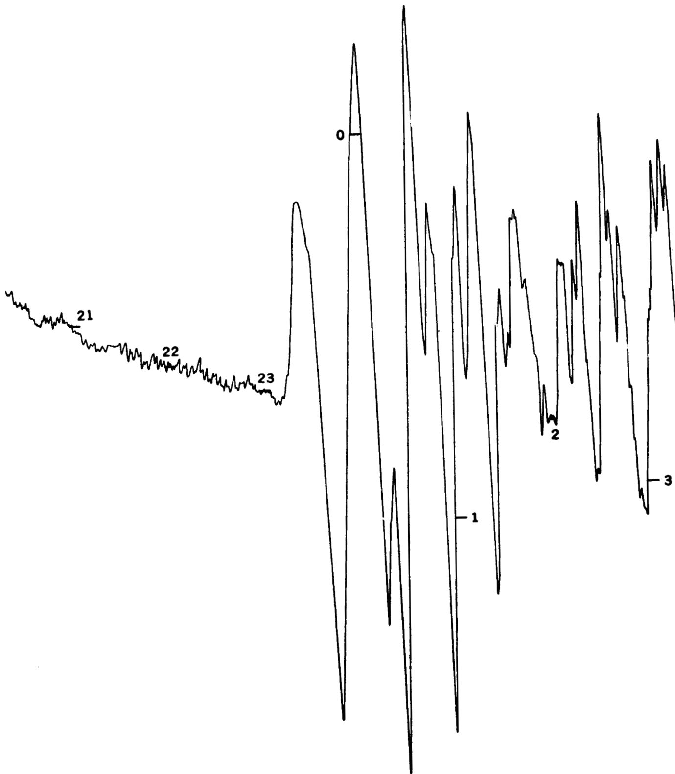
Figure 18. - Honolulu tide record showing tsunami produced by earthquake off Kamchatka at 1658Z, 4 November 1952.
