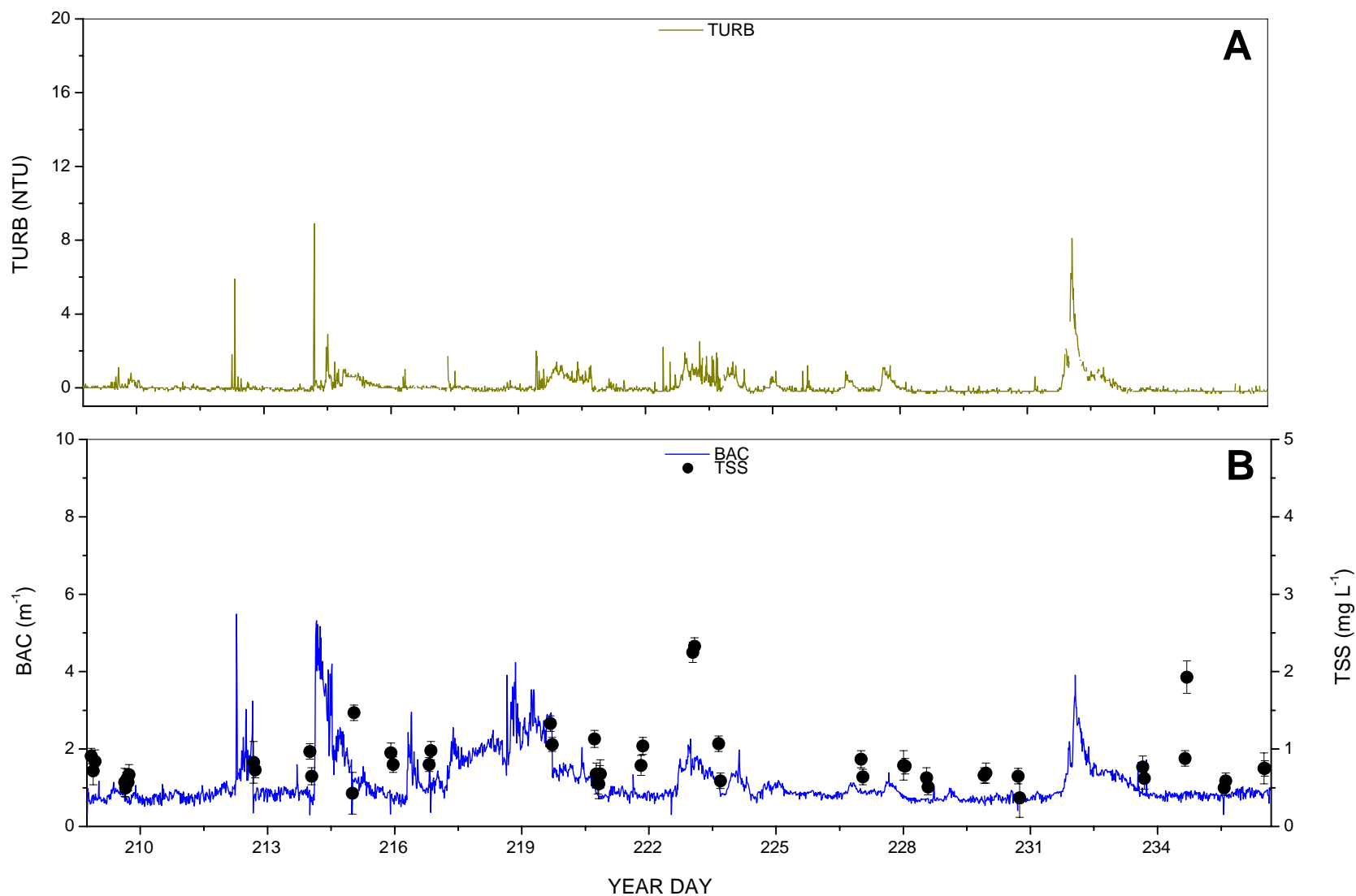
Figure 19. Grand Traverse Bay, Lake Michigan, MI. A) Turbidity (TURB; Nephelometric Turbidity Units) measured by the YSI 6600 EDS Sonde; B) Beam Attenuation Coefficient (BAC) measured by an in situ transmissometer, and total suspended solids (TSS).
