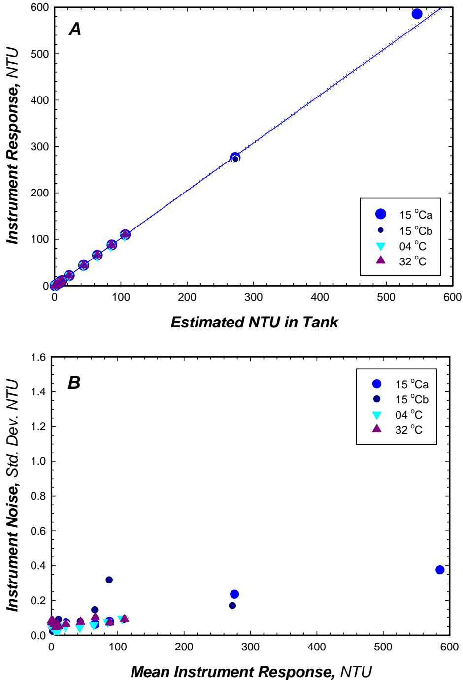
Figure 1. YSI 6600 Sonde equipped with a 6136 turbidity sensor. Signal and instrument noise in response to increasing turbidity derived from SDVB added to filtered deionized water at three test temperatures. (A) Mean detector response to sequential additions of known SDVB concentrations. Instrument response over a turbidity range normally observed in natural waters (0-100 NTU) was modeled by linear regression. Modeled response at 15°C, with 99% confidence intervals (dotted lines): NTU_{instru} = 1.029NTU_{SDVB} - 0.827 , r^2 = 0.999 , demonstrates response is linear through 300 NTU SDVB. Detector response was unaffected by the ambient temperatures tested. (B) Signal noise (s.d.) ranged from <0.1 to 40% of measured signal in the presence of SDVB and increased with measured turbidity.
