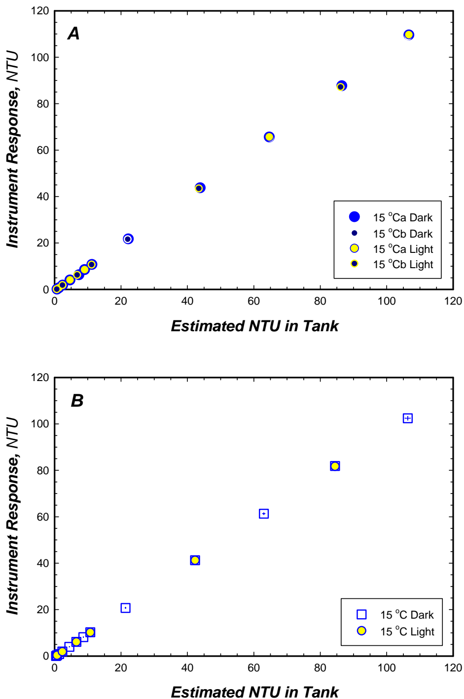
Figure 3. Effects of downwelling irradiance on turbidity measurement by the YSI 6600 Sonde with 6136 Turbidity sensor . Surface irradiance applied at each indicated test concentration using a bank of three 500W halogen lamps. E_0 : 400-500 \mu\text{mol quanta m}^{-2} \text{s}^{-1} measured using a Licor 190S detector. (A) Mean detector response to sequential additions of known SDVB concentrations. (B) Mean detector response to sequential additions of known Formazin concentrations. Exposure to down-welling irradiance did not have a significant impact on instrument response under these test conditions.
