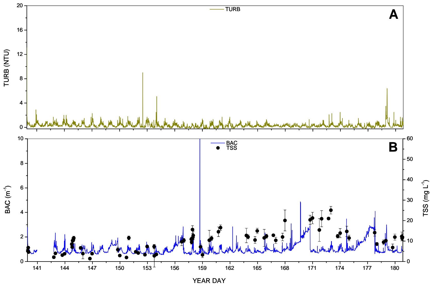
Figure 13. Kaneohe Bay, HI. A) Turbidity (TURB; Nephelometric Turbidity Units) measured by the YSI 6600 EDS Sonde; B) Beam Attenuation Coefficient (BAC) measured by an in situ transmissometer, and total suspended solids (TSS).
