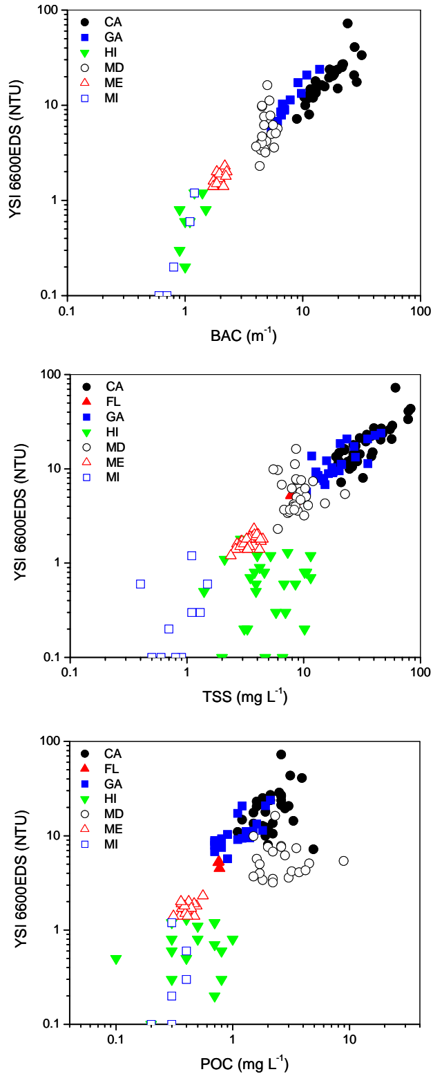
Figure 21. YSI 6600EDS Sonde turbidity data (in Nephelometric Turbidity Units) plotted against Beam Attenuation Coefficients (BAC), collected total suspended solids (TSS) and particulate organic carbon (POC).
