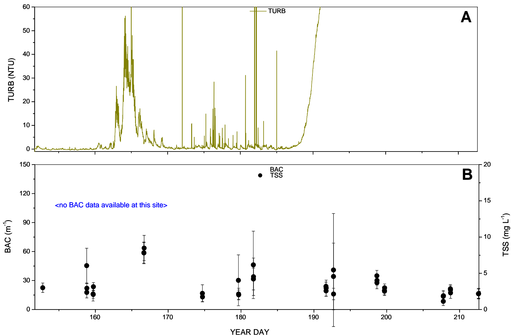
Figure 9. Offshore of Tampa Bay, FL. A) Turbidity (TURB; Nephelometric Turbidity Units) measured by the YSI 6600 EDS Sonde; B) Beam Attenuation Coefficient (BAC) measured by an in situ transmissometer, and total suspended solids (TSS).
