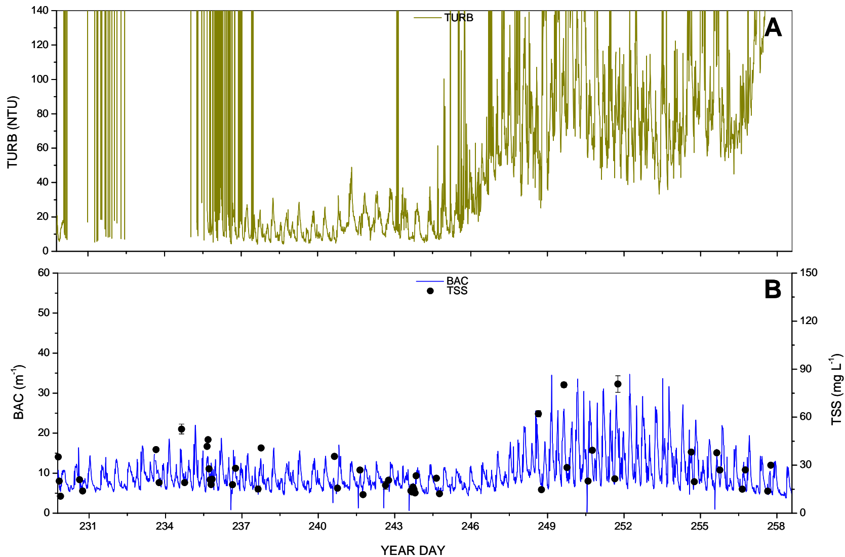
Figure 11. Skidaway Island, GA. A) Turbidity (TURB; Nephelometric Turbidity Units) measured by the YSI 6600 EDS Sonde; B) Beam Attenuation Coefficient (BAC) measured by an in situ transmissometer, and total suspended solids (TSS).
