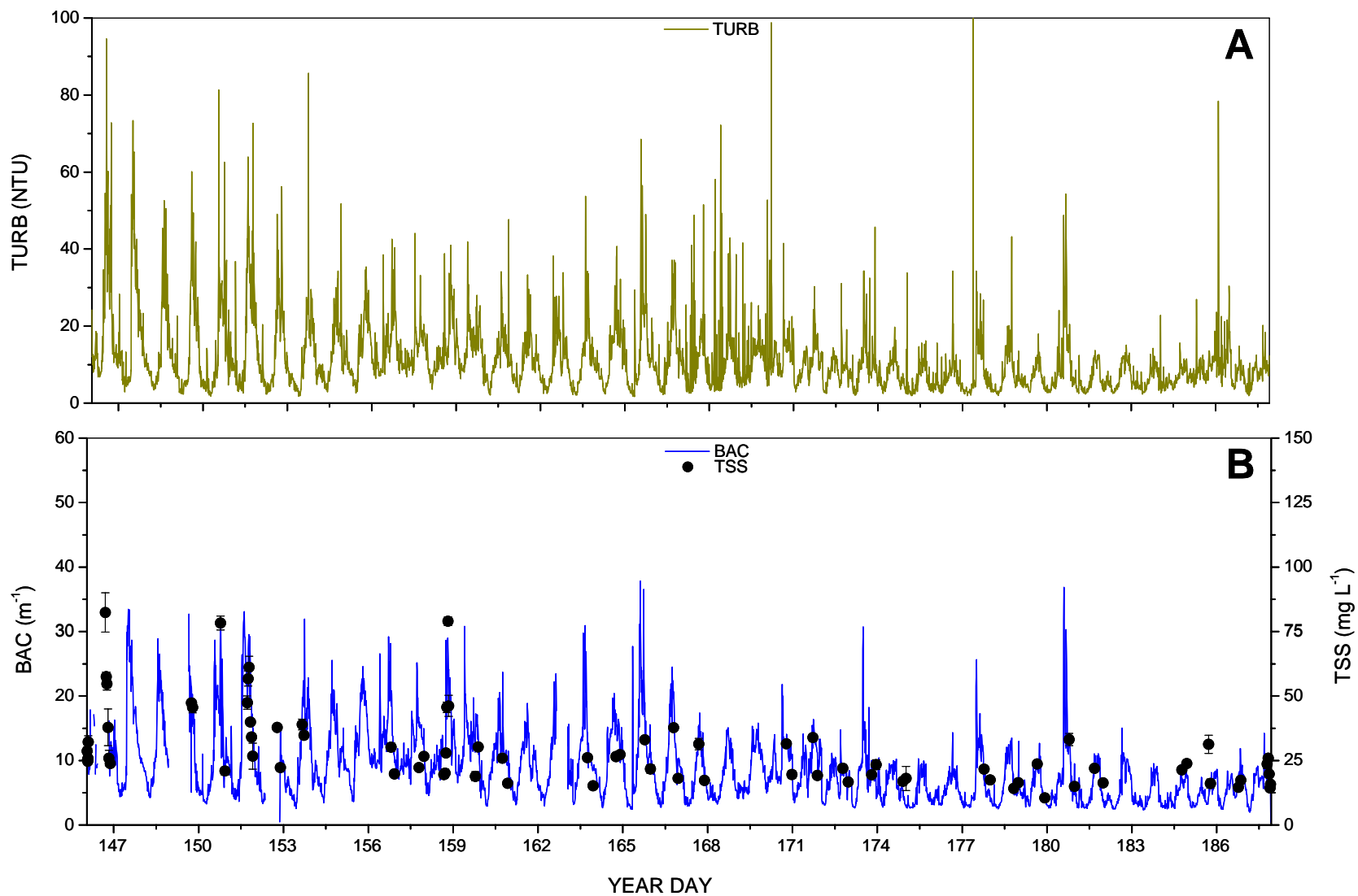
Figure 7. Moss Landing Harbor, CA. A) Turbidity (TURB; Nephelometric Turbidity Units) measured by the YSI 6600 EDS Sonde; B) Beam Attenuation Coefficient (BAC) measured by an in situ transmissometer, and total suspended solids (TSS).
