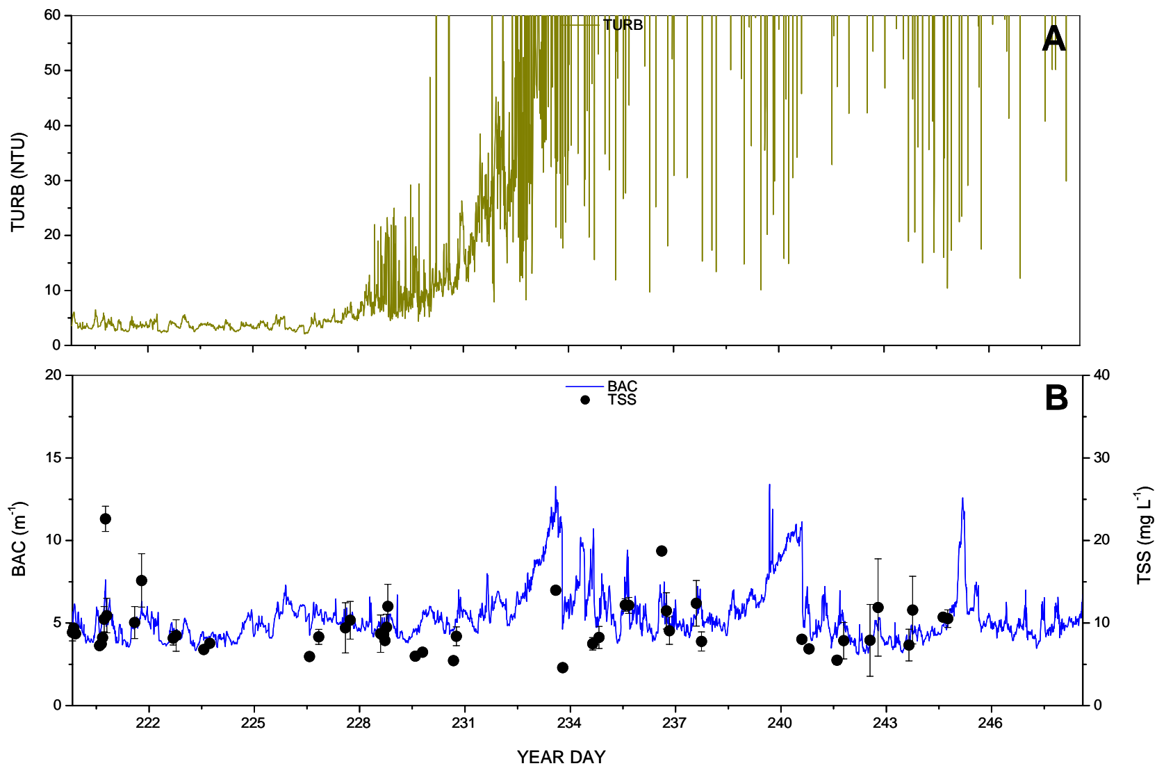
Figure 15. Chesapeake Bay, MD. A) Turbidity (TURB; Nephelometric Turbidity Units) measured by the YSI 6600 EDS Sonde; B) Beam Attenuation Coefficient (BAC) measured by an in situ transmissometer, and total suspended solids (TSS).
