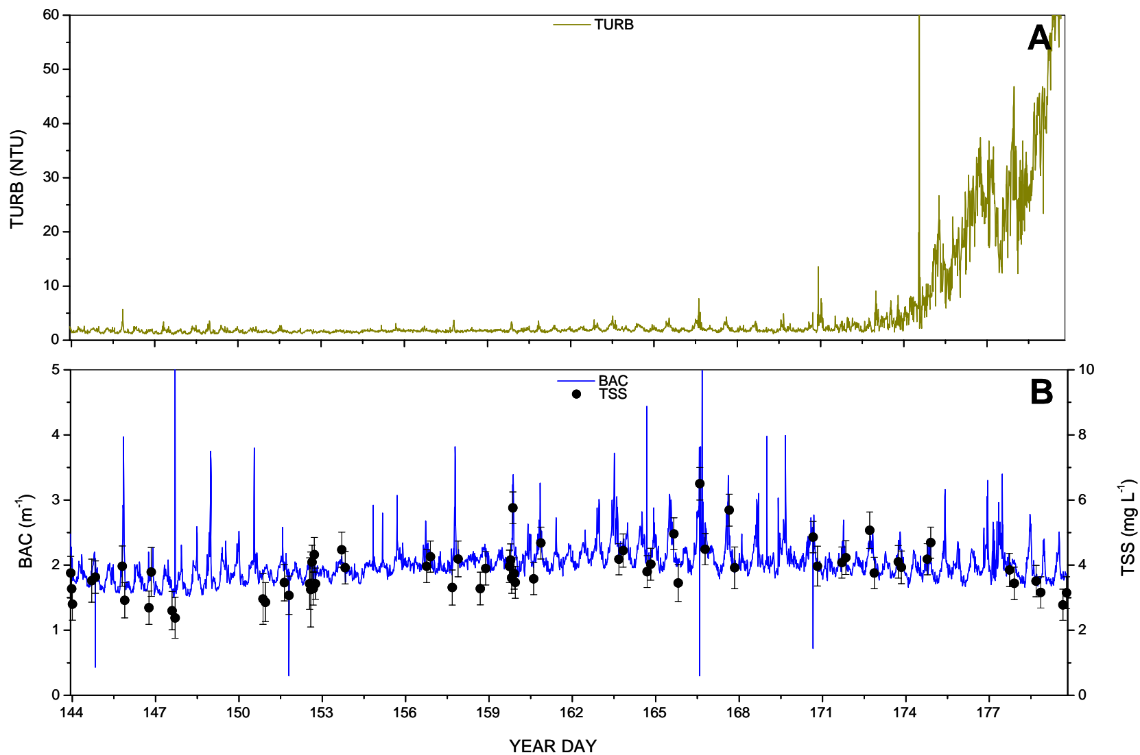
Figure 17. Damariscotta River Estuary, ME. A) Turbidity (TURB: Nephelometric Turbidity Units) measured by the YSI 6600 EDS Sonde; B) Beam Attenuation Coefficient (BAC) measured by an in situ transmissometer, and total suspended solids (TSS).
