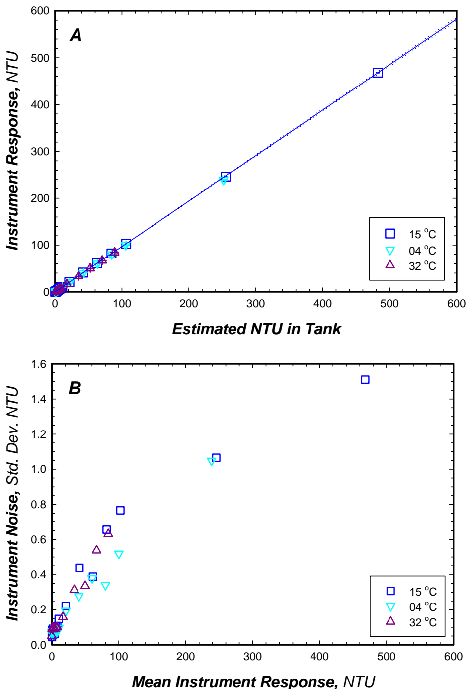
Figure 2. YSI 6600 Sonde equipped with a 6136 turbidity sensor. Signal and instrument noise in response to increasing turbidity derived from Formazin added to filtered deionized water at three test temperatures. (A) Mean detector response to sequential additions of known Formazin concentrations. Instrument response over a turbidity range normally observed in natural waters (0-100 NTU) was modeled by linear regression. Modeled response at 15°C, with 99% confidence intervals (dotted lines): NTU_{instru} = 0.971NTU_{FRMZ} - 0.277 , r^2 = 0.999 , demonstrates response is linear through at least 500 NTU Frmz. Detector response was unaffected by the ambient temperatures tested. (B) Signal noise (s.d.) ranged from 0.3 to 50% of measured signal and was independent of temperature. The monotonic increase in signal s.d. with Formazin turbidity, likely results from detection of particle aggregates in suspension.
